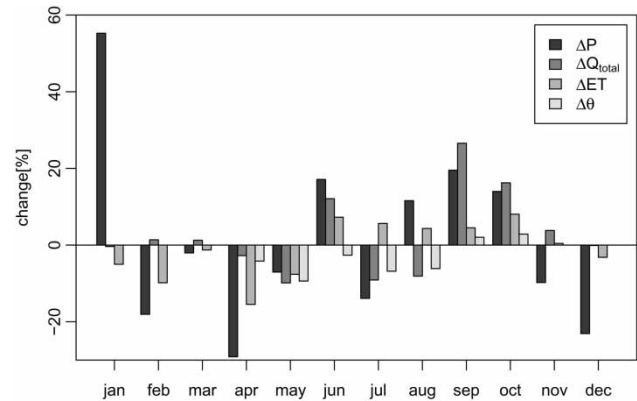
Figure 9 | Monthly mean changes in precipitation (P), runoff (Q total ), evapotranspiration (ET) and soil moisture (θ) (%) (2030–2039 vs 1991–2000, entire Volta Basin).
