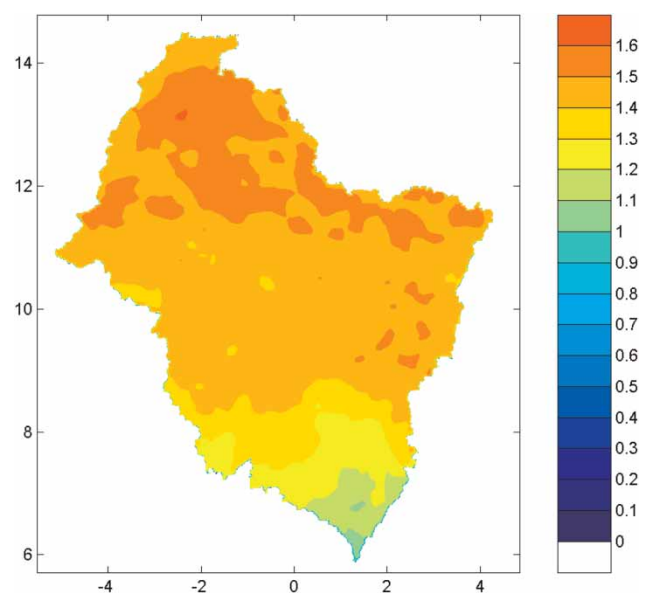
Figure 5 | Annual mean temperature change (°C) (2030–2039 vs 1991–2000).
