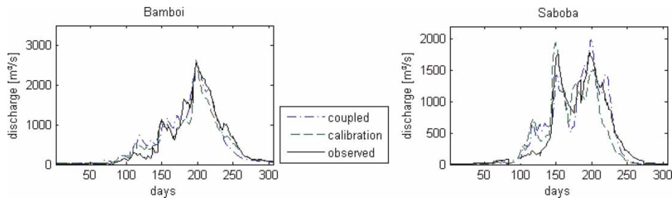
Figure 4 | Observed and simulated discharge ( Q_{\text{total}} ) ( \text{m}^3 \text{s}^{-1} ) (calibration run and joint MM5–WaSiM run), left: Bamboi, right: Saboba, 1968.
