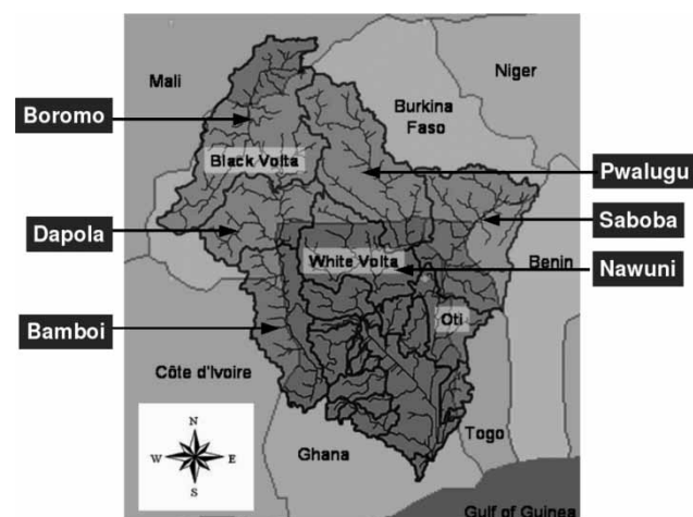
Figure 2 | WaSiM set-up: subcatchments and flow net structure.
