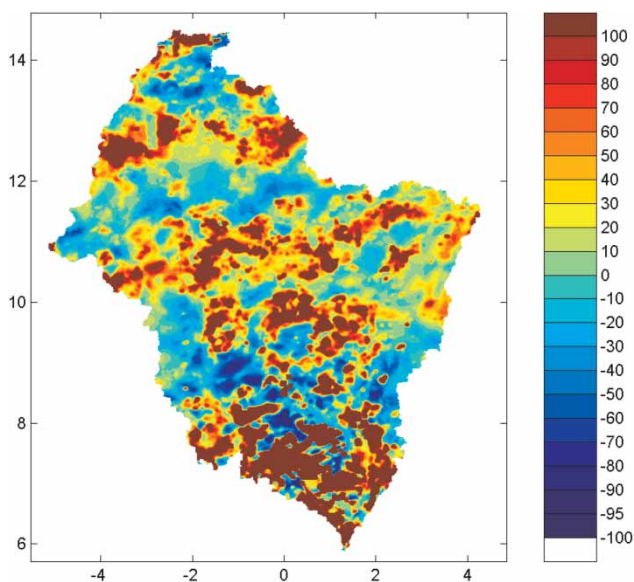
Figure 10 | Annual mean total runoff change (%) (2030–2039 vs 1991–2000).
