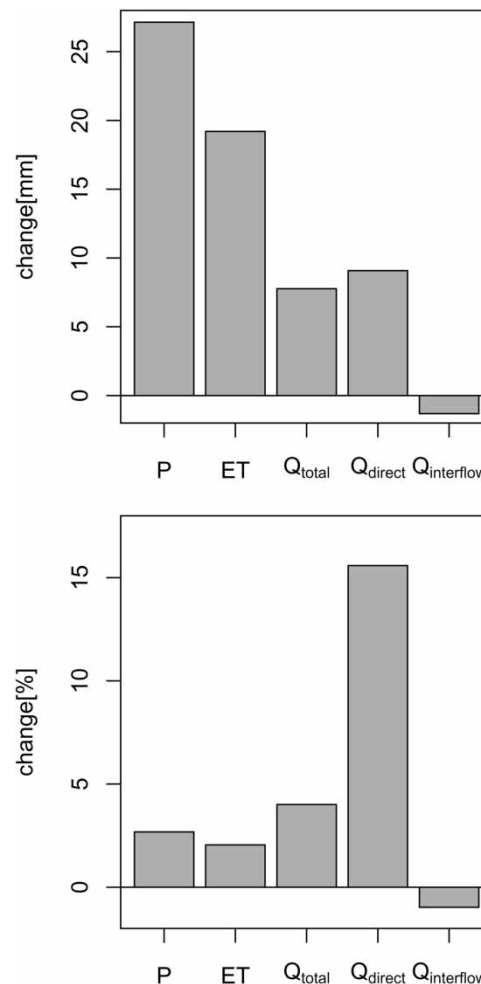
Figure 7 | Mean annual changes (2030–2039 vs 1991–2000) in the most important hydrological variables for the entire Volta Basin. Top: absolute values (mm), bottom: relative to (1991–2000) (%).
