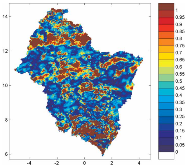
Figure 12 | Signal-to-noise ratio ( SN ) for total runoff.
