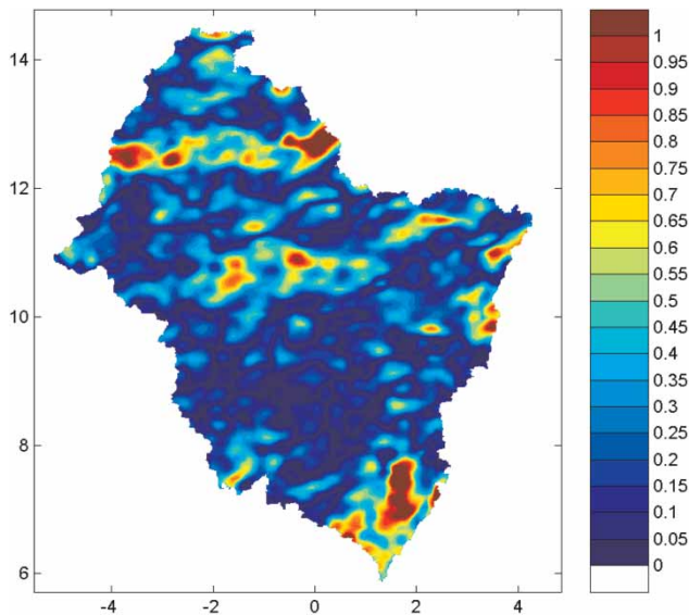
Figure 11 | Signal-to-noise ratio ( SN ) for precipitation.
