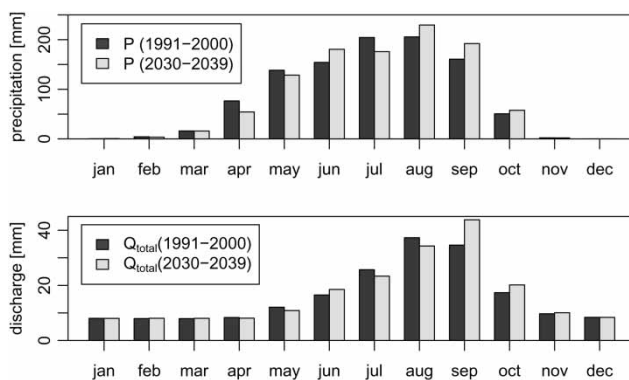
Figure 8 | Monthly decadal mean amounts of precipitation (top) and discharge (bottom) (mm) (1991–2000 and 2030–2039, entire Volta Basin).
