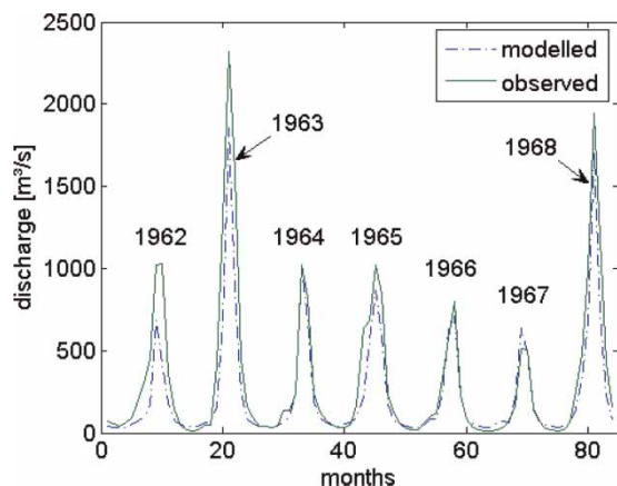
Figure 3 | Monthly values of observed and simulated discharge ( \text{m}^3 \text{s}^{-1} ) for the years 1962–1969, Bamboi.
