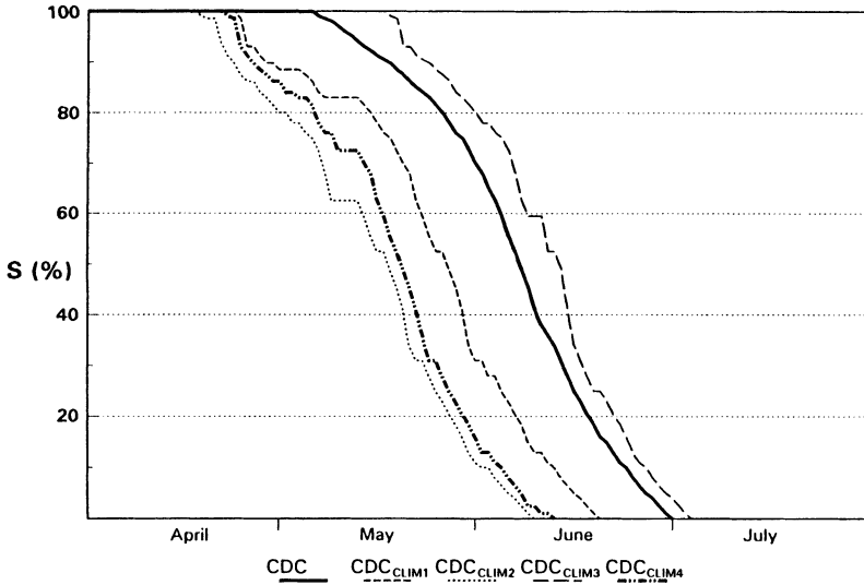
Fig. 7. Comparison of the conventional depletion curve (CDC) for 1979 in elevation zone B (2,926-3,353 m a.s.l.) of the Rio Grande basin, Colorado with curves for four examples of changed climate as generated by the Snowmelt-Runoff Model computer program: CDC_{CLIM1} ( T + 2^{\circ}C ), CDC_{CLIM2} ( T + 4^{\circ}C ), CDC_{CLIM3} ( P \times 2 ), and CDC_{CLIM4} ( T + 4^{\circ}C , P \times 2 ).
