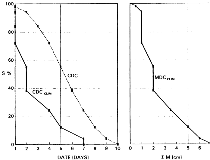
Fig. 5. Depletion curves of the snow coverage in the present climate (CDC) and in a changed climate ( T + 1^{\circ}\text{C} , P \times 2 ), CDC CLIM , as derived from MDC CLIM .
