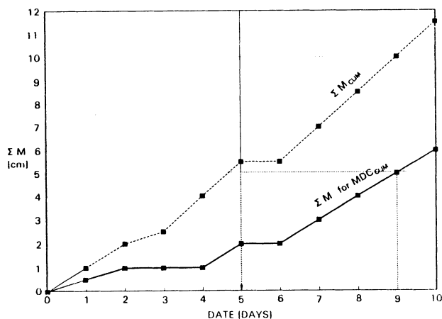
Fig. 2. Graphical determination of time shifting of snow covered area by a changed climate ( T + 1^{\circ}\text{C} ): In the present climate, a cumulative snowmelt depth of 5 cm is reached on day 9 (with new snow falls adjusted to T + 1^{\circ}\text{C} ), in the changed climate 5 cm is reached already on day 5.
