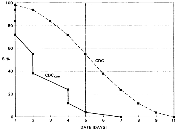
Fig. 3. Depletion curves of the snow coverage in the present climate (CDC) and in a changed climate ( T + 1^\circ ), CDC_{CLIM} .
