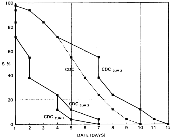
Fig. 6. Comparison of the depletion curve of the snow coverage in the present climate (CDC) with curves for three examples of a changed climate: CDC_{CLIM1} ( T + 1^\circ ), CDC_{CLIM2} ( P \times 2 ) and CDC_{CLIM3} ( T + 1^\circ , P \times 2 ).
