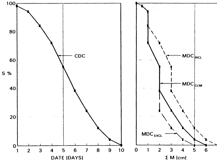
Fig. 1. Example of a conventional depletion curve of snow covered areas, CDC, and auxiliary curves for evaluating the effect of a changed climate: Modified depletion curves including and excluding the effect of new snow, MDC_{INCL} and MDC_{EXCL} , and the modified depletion curve for a changed climate ( T + 1^{\circ}C ), MDC_{CLIM} .
