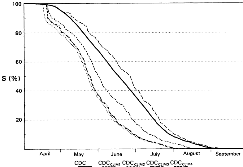
Fig. 8. Comparison of the conventional depletion curve (CDC) for 1981 in elevation zone B (1,200-1,800 m a.s.l.) of the Illecillewaet River basin, British Columbia with curves for four examples of changed climate as generated by the Snowmelt-Runoff Model computer program: CDC_{CLIM1} ( T + 2^{\circ}C ), CDC_{CLIM2} ( T + 4^{\circ}C ), CDC_{CLIM3} ( P \times 2 ), and CDC_{CLIM4} ( T + 4^{\circ}C , P \times 2 ).
