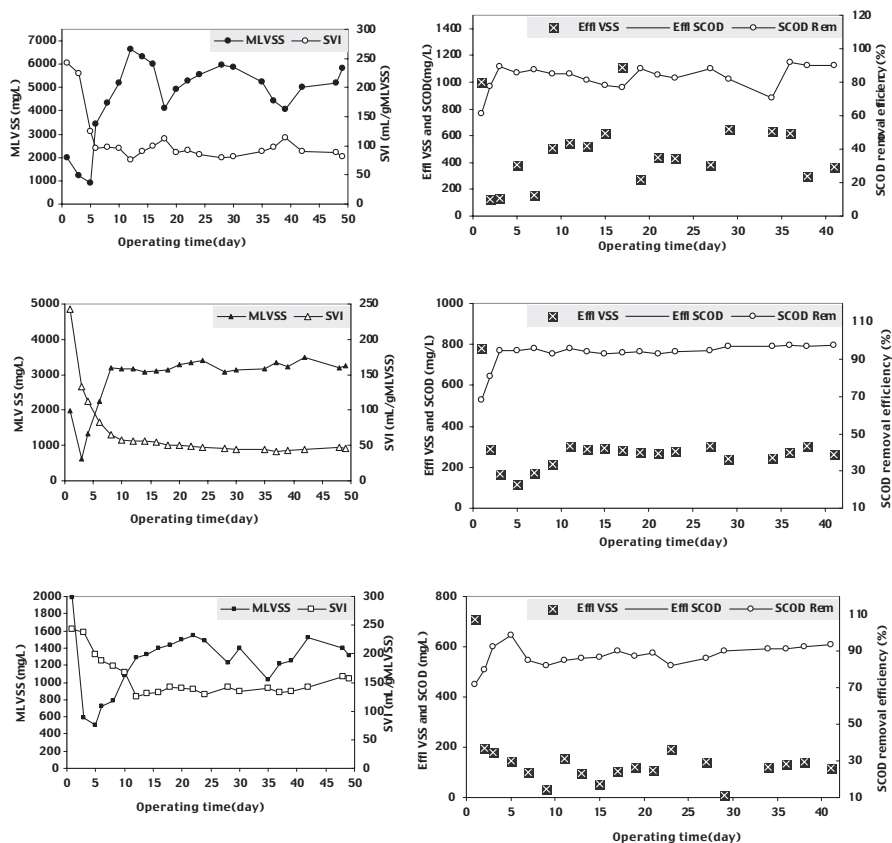
Figure 1 Reactor performance under different OLR. Top, middle and bottom, the applied OLR are 8, 4 and 2 kg COD·(m 3 ·d) -1 respectively
