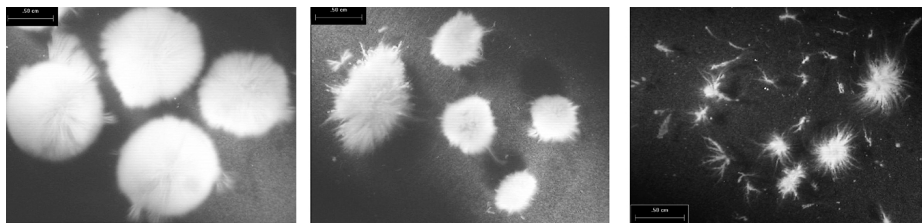
Figure 2 Stereomicroscopic pictures of aerobic granules. From A to C, the applied OLR are 8, 4 and 1 kg COD ·(m 3 ·d) -1 respectively
