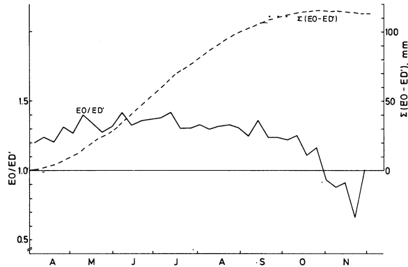
Fig. 5. Evaporation ratio and accumulated difference for the evaporimeters EO and ED. Averaged for the years 1964-1976.
