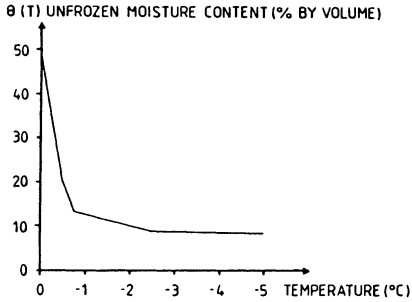
Fig. 4. Unfrozen moisture content and hydraulic conductivity as a function of the temperature below freezing point (0°C) for Bensby Silt. The relationships are estimated from experimental data measured by Burt and Williams (1976).
