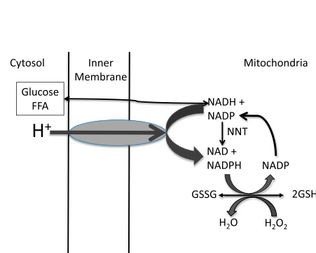
Figure 4 —Communication among cellular redox and ROS systems. NADH, generated from metabolism, can be used to regulate the NADPH/NADP and GSH/GSSG redox states via the NNT. The proton-translocating NNT reduces NADP by NADH and is an inner membrane protein utilizing the electrochemical proton gradient for NADPH generation. This enzyme has an important physiological role in the maintenance of reduced glutathione, essential for scavenging reactive oxygen. ROS stimulates scavenging activities using NADPH and increasing flux through NNT.
