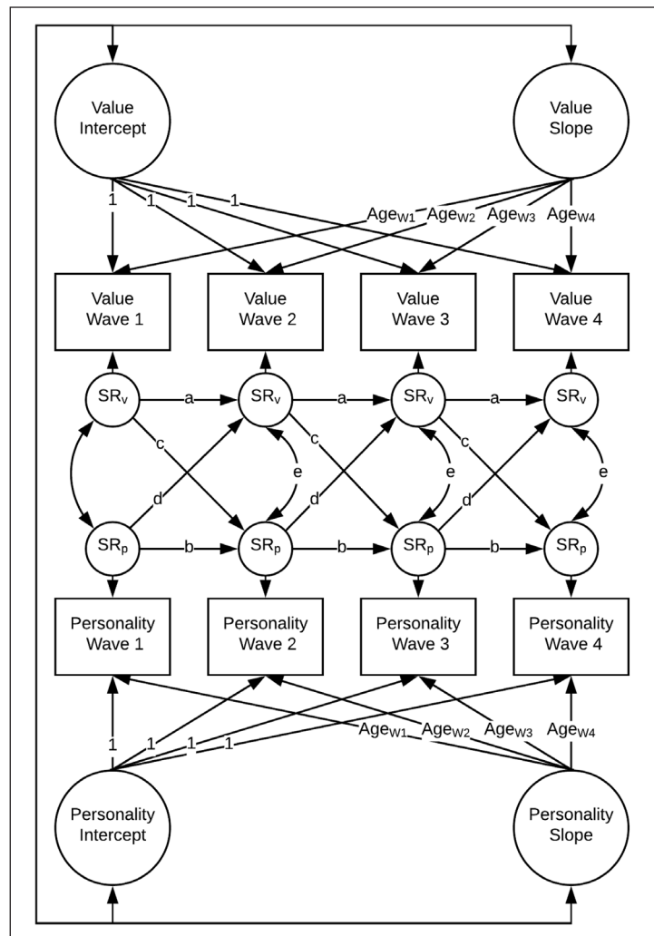
Figure 1: Diagram representing the Latent Curve Model with Structured Residuals. Manifest variables are computed scale scores for each value and personality variable. Latent structured residual factors (SR) have loadings fixed to 1. Autoregressive paths are fixed to be equal between waves for the value (a) and personality (b) variables. Cross-lagged paths are also fixed to equality both for personality SRs regressed on value SRs (c) and value SRs regressed on personality SRs (d). The within-wave correlations of SR residuals are fixed to equality for the last three waves (e).
