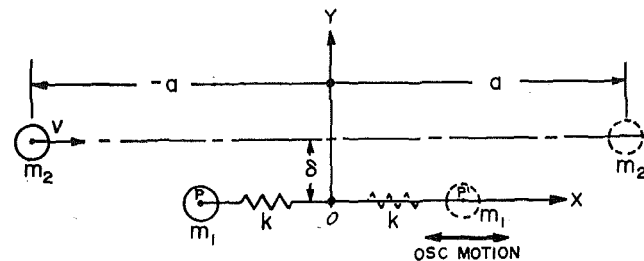
Fig. 2 Atomic model
