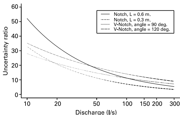
Figure 1 Uncertainty ratio plots for two thin plate notch weirs (crest lengths 0.3 and 0.6 m) and two thin plate v-notch weirs (angles 90^\circ and 120^\circ )
