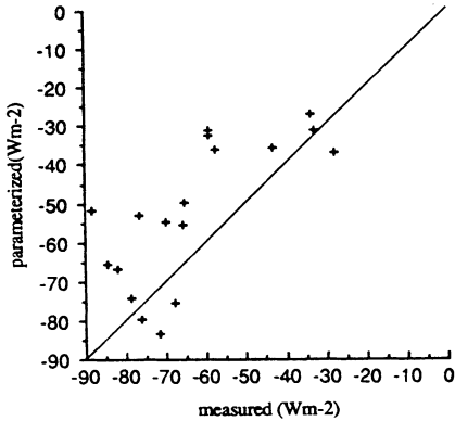
Fig. 3. Daily mean long-wave net radiation: Measured values compared with parameterization (1-18 May 1992).
