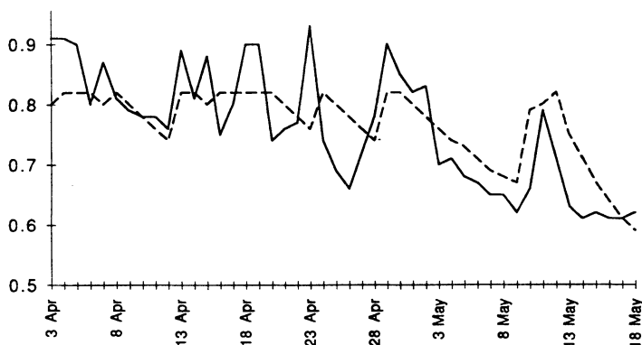
Fig. 2. Daily mean albedo measured (solid line) and parameterized (dashed line). The parameterization slightly underestimates the albedo during the premelt period and overestimates it during the melt period.
