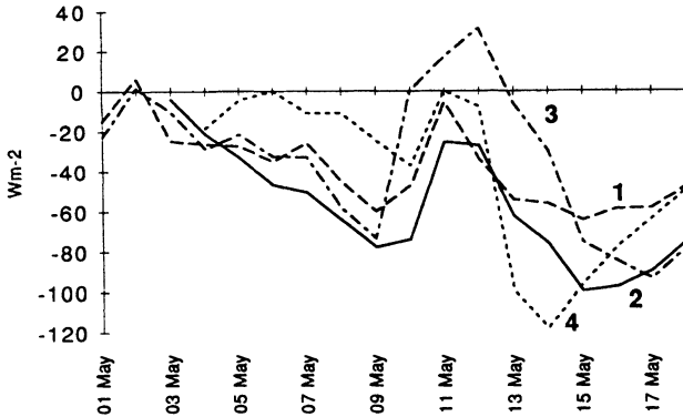
Fig. 7. Melt energy at Weissfluhjoch calculated using different methods: 1) Measured energy balance, 2) Measured runoff, 3) Parameterized energy balance, 4) Degree-day.
