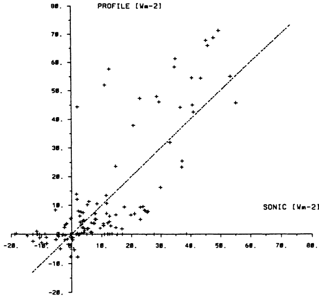
Fig. 5. Sensible heat flux (30 min means) derived from 4-level profile measurements (vertical axis) compared with eddy correlation (horizontal axis). Data from 21 March, 24 April, 11 May and 12 May 1993 were compared.
