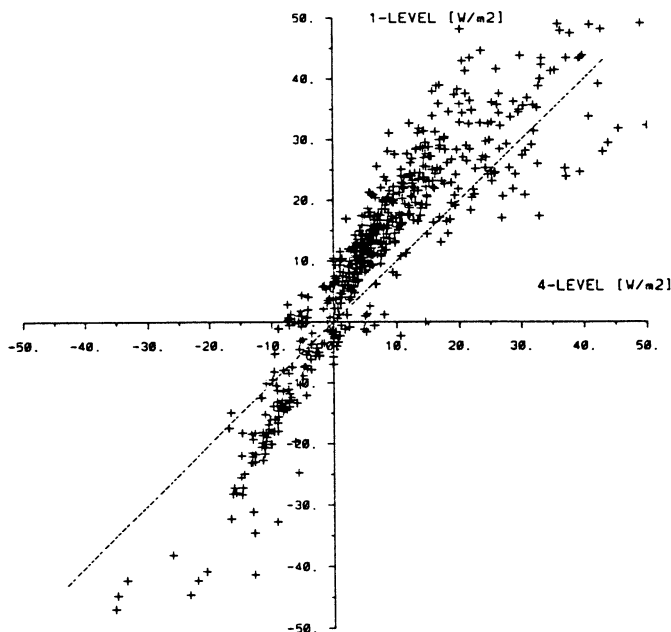
Fig. 6. Sensible heat flux (30 min means) derived from 4-level profile measurements compared to a bulk approach for wind speeds > 2 m/s. May and June 1993.
