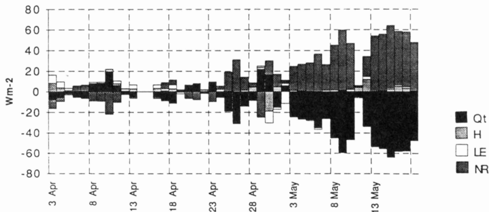
Fig. 1. Energy Balance at Weissfluhjoch (2,540 m) in spring 1992 as derived from measurements. Q_t = total heat flux passing the surface; H = sensible heat flux; LE = latent heat flux; NR = net radiation.
