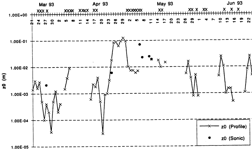
Fig. 4. Daily mean roughness lengths for momentum calculated from 4-level profile measurements or from sonic anemometer measurements in near neutral conditions. A daily average value was calculated if more than 4 runs were available during the respective day. The 'X' on the time axis indicates snowfall events ( > 2 cm).
