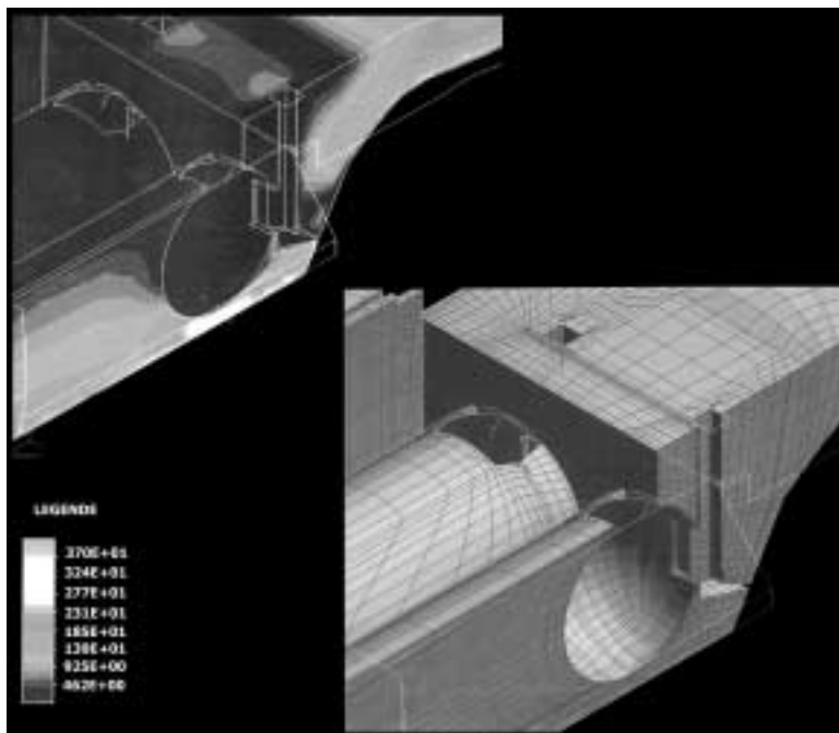
Figure 5 Flow pattern around the balls
