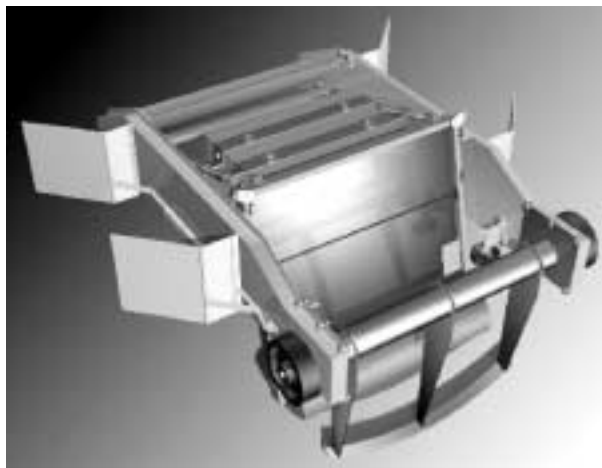
Figure 7 Physical model of the new flushing unit on the scale 1:5
