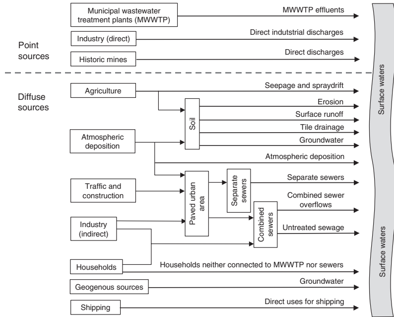
Figure 2 Sources and pathways of heavy metal input into river systems (Fuchs et al. , 2002)
