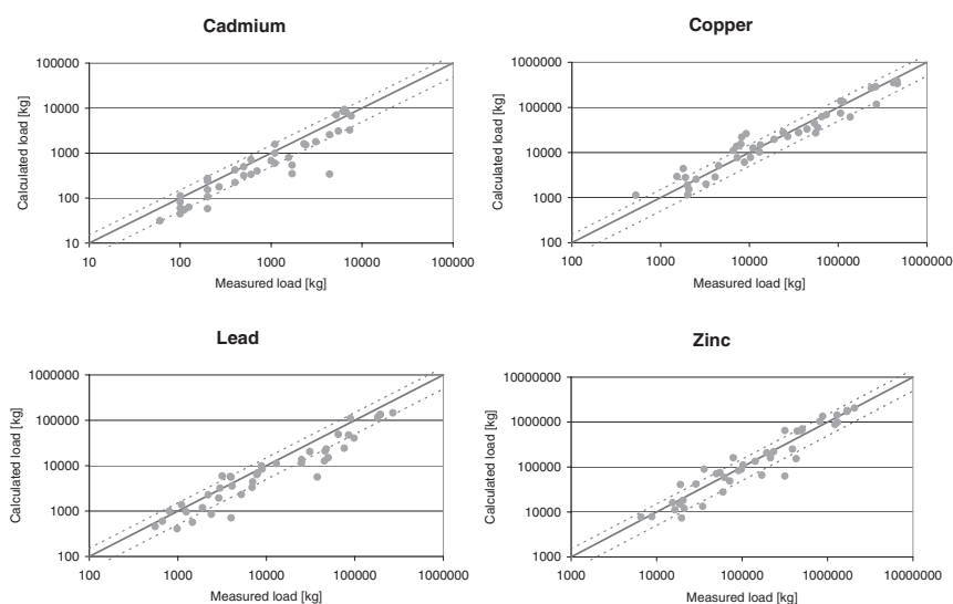
Figure 4 Relationship between measured and simulated heavy metal loads (estimated heavy metal emission minus losses according to retention processes) for several monitoring stations of German river basins
