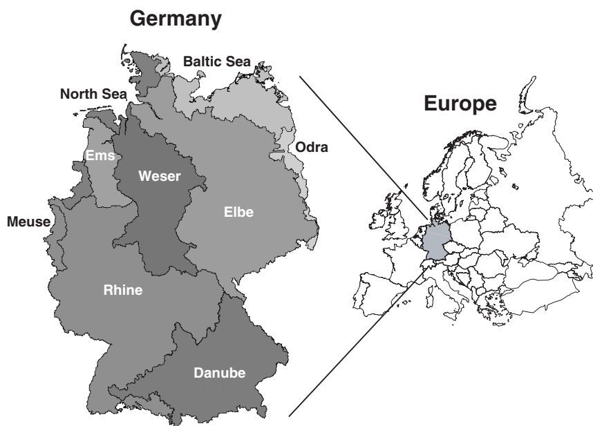
Figure 1 Geographical overview of the large German river basins
