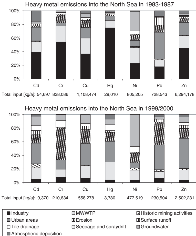
Figure 3 Heavy metal emissions into the North Sea [kg/a]
