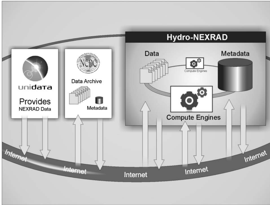
Figure 2 | A general schematic of Hydro-NEXRAD functionality. Basic data are provided in two modes: (1) in real-time from Unidata and (2) by accessing the NCDC archives. Both data acquisition and products dissemination occur over the Internet.
