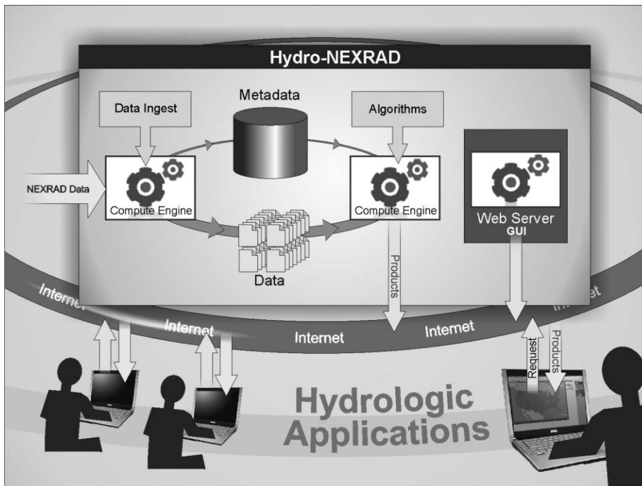
Figure 3 | Information technology elements of Hydro-NEXRAD. Shown are (1) file servers' dedicated storage of the data and the database; (2) compute servers dedicated to ingesting the data and calculating the metadata, computation of the products and running various utilities and (3) web servers to provide web services via graphical user interface and a mapserver.
