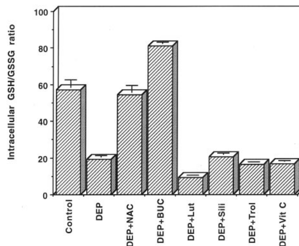
FIGURE 1. In vitro exposure to an organic DEP extract induces a decrease in the GSH:GSSG ratio in RAW 264.7 cells. Cells were treated with 50 μg/ml DEP extract in the presence or the absence of the following antioxidants for 5 h: NAC, 20 mM; BUC, 5 mM; luteolin (Lut), 50 μg/ml; silibinin (sili), 25 μg/ml; trolox (water-soluble vitamin E), 1 μM; and vitamin C (Vit C), 100 μM. Cell lysates were used to measure the cellular GSH:GSSG ratios in duplicate, as described in Materials and Methods . Values are the mean ± SEM. This experiment was reproduced once, with similar results.
