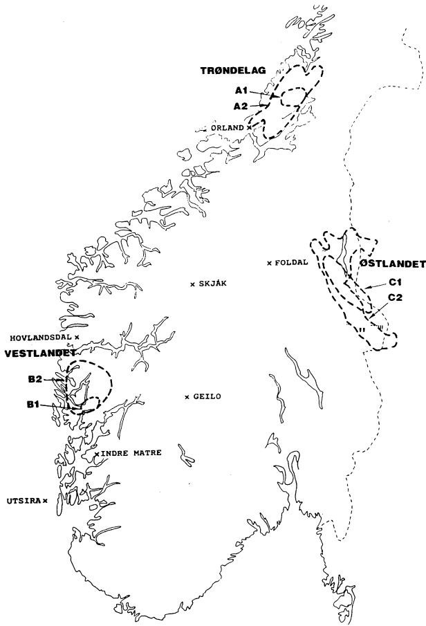
Fig. 5. Basins (A,B,C) where PMP is estimated. Locations mentioned in the text are also indicated.
