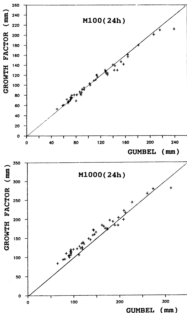
Fig. 4. Scatter diagram for »Growth-Factor« and Gumbel estimates for 24-hour rainfall with return periods: a) 100 years and b) 1,000 years.
