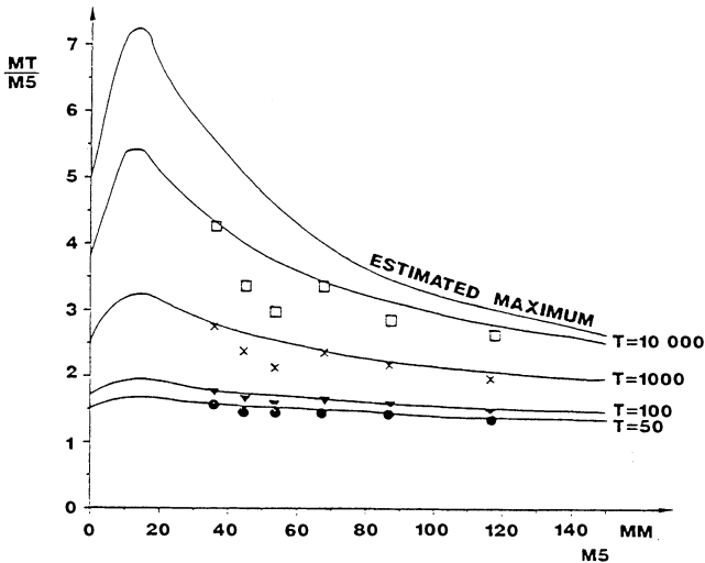
Fig. 3. Growth-Factors MT/M5 as a function of the M5 -value. Solid curves are ratios from Scotland/Northern Ireland (NERC 1975), whereas the point values are corresponding Norwegian values for return periods ( T ) of 50 ( \bullet ), 100 ( \blacktriangledown ), 1,000 ( \times ) and 10,000 ( \square ) years.
