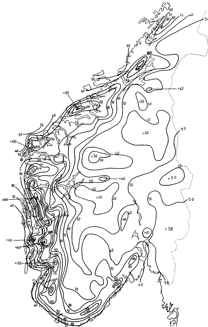
Fig. 2. Estimated 24-hour rainfall values (mm) with 5-year return period.
