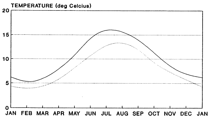
Fig. 6. Maximum 1-day dewpoints at sea level (1,000 hPa) for basin A1 (solid curve). Mean monthly sea temperature (dashed curve) for a lighthouse 60 km southwest of the basin is also indicated.
