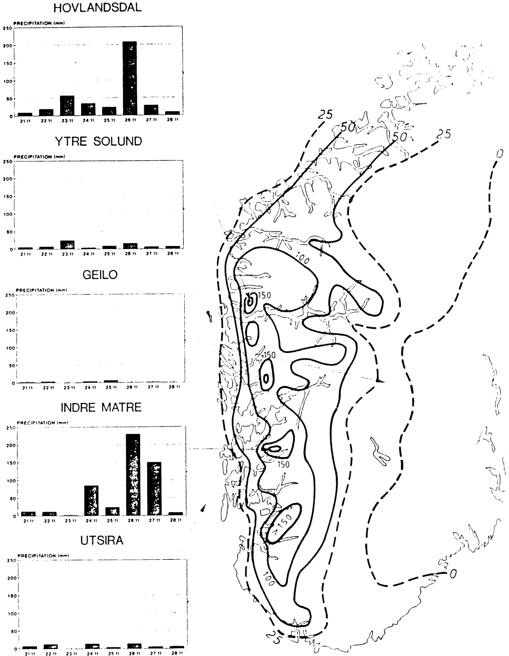
Fig. 1. 1-day precipitation (mm) in Western Norway, 26 November, 1940. Diagrams to the left illustrate daily rainfall amounts at 5 stations for the period 21-28 November, 1940.
