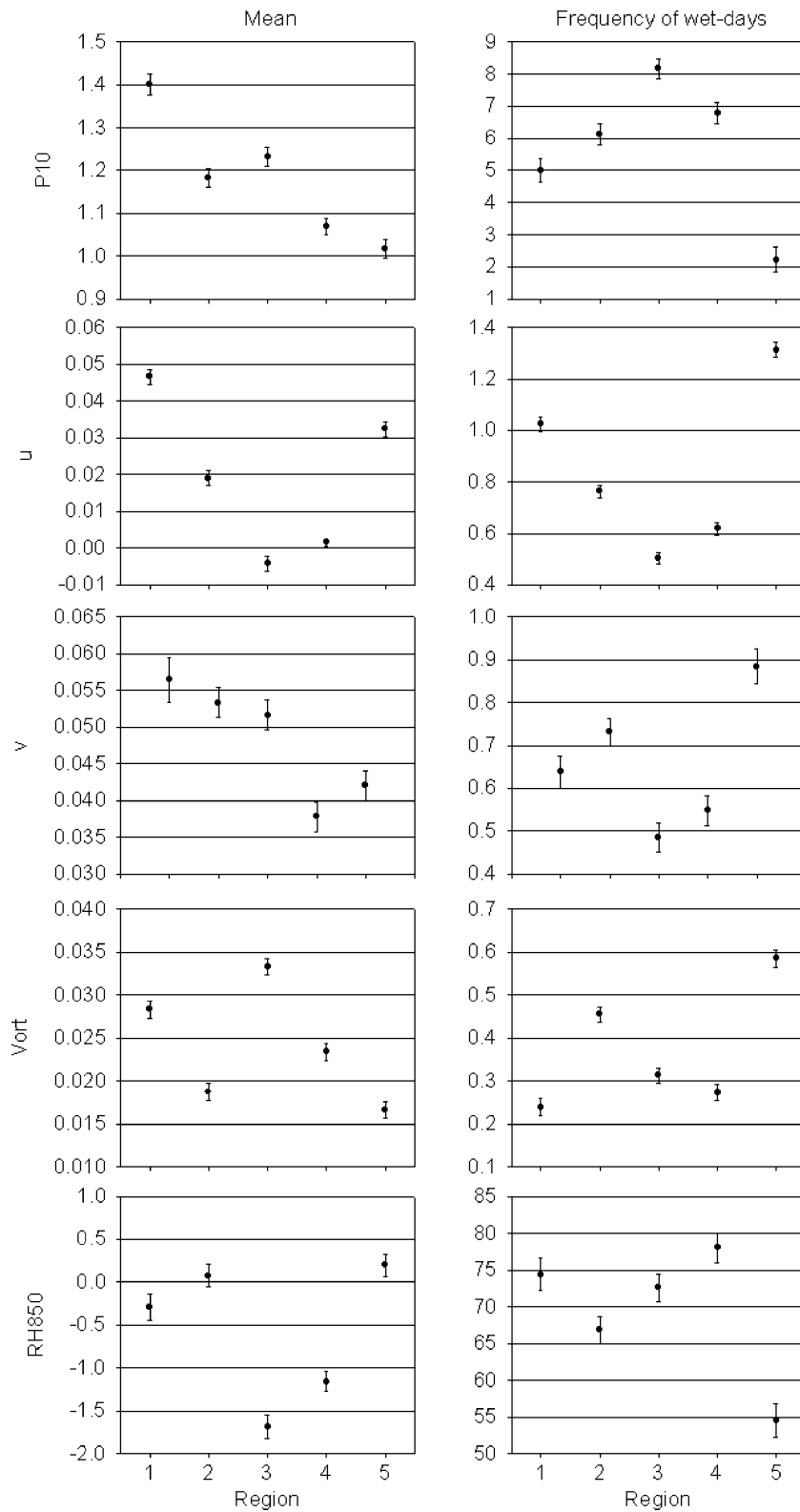
Figure 2 Standardised regression coefficients of the winter downscaling models with 95% confidence intervals
