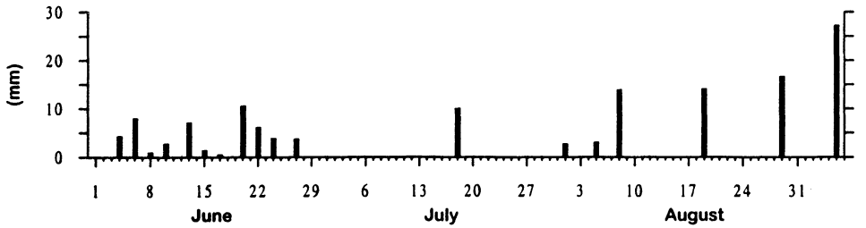
Fig. 5. Precipitation (mm), Ryggmossen 1994.
