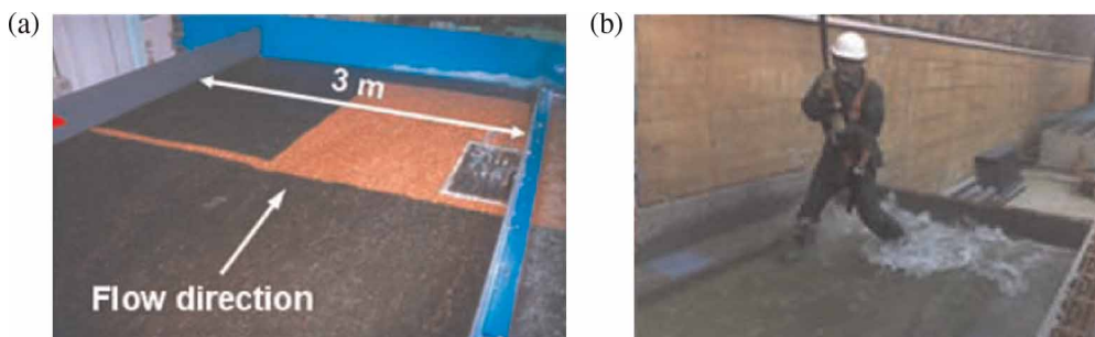
Figure 1 | (a) UPC platform for testing inlets and (b) human subject during the tests in the hydraulic department of the UPC.
