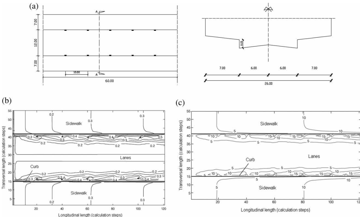
Figure 2 | (a) Geometric characteristic of the street reach analyzed; (b) map of the flow velocities (m/s) and (c) map of the flow depths (mm), on a flat street. The water is flowing left to right.
