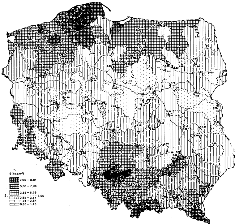
Fig. 4. Groundwater runoff modulus.
