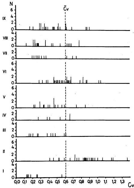
(c) Coefficient of groundwater runoff variation.
