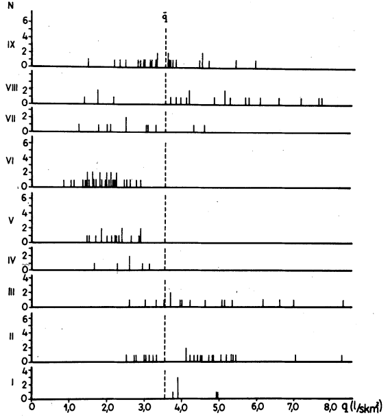
(b) Groundwater unit runoff modulus.
