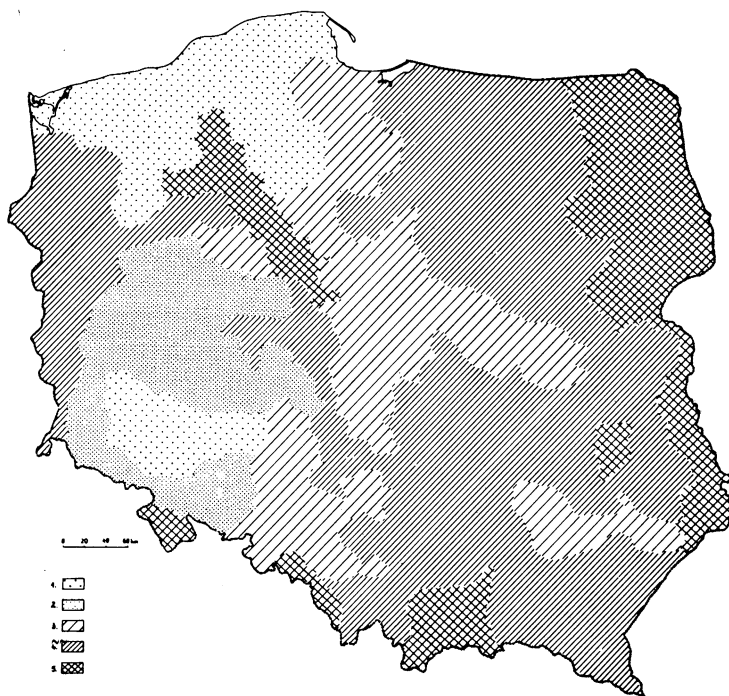
Fig. 5. Typical time of underground floods.
