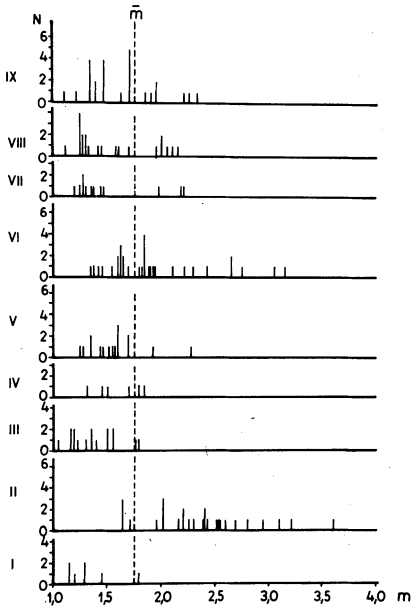
(a) Storage capacity of catchment basin.
