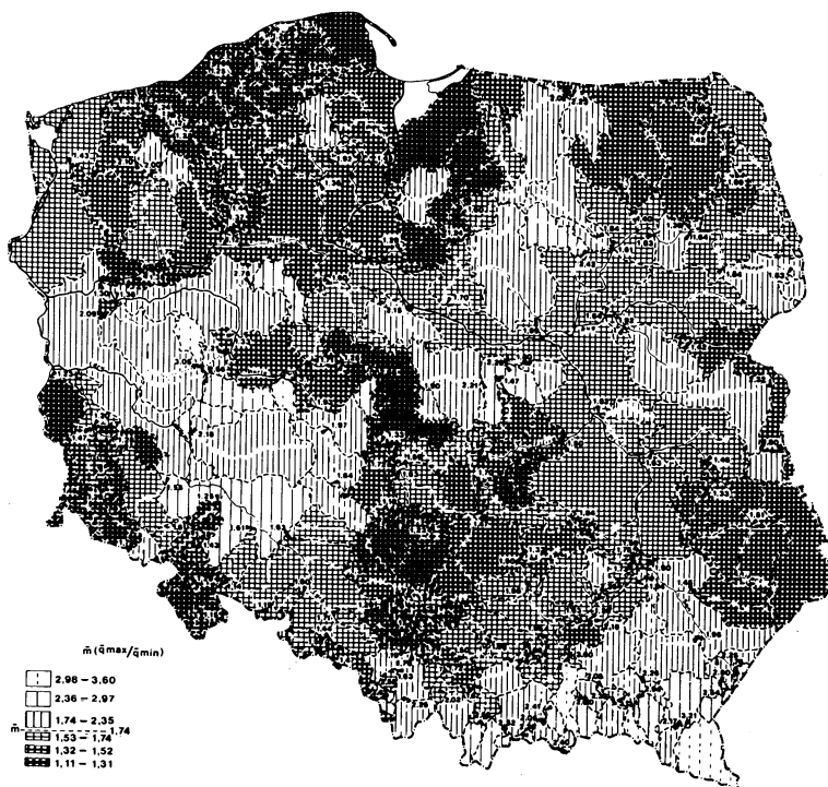
Fig. 3. Storage capacity of catchment basin.
