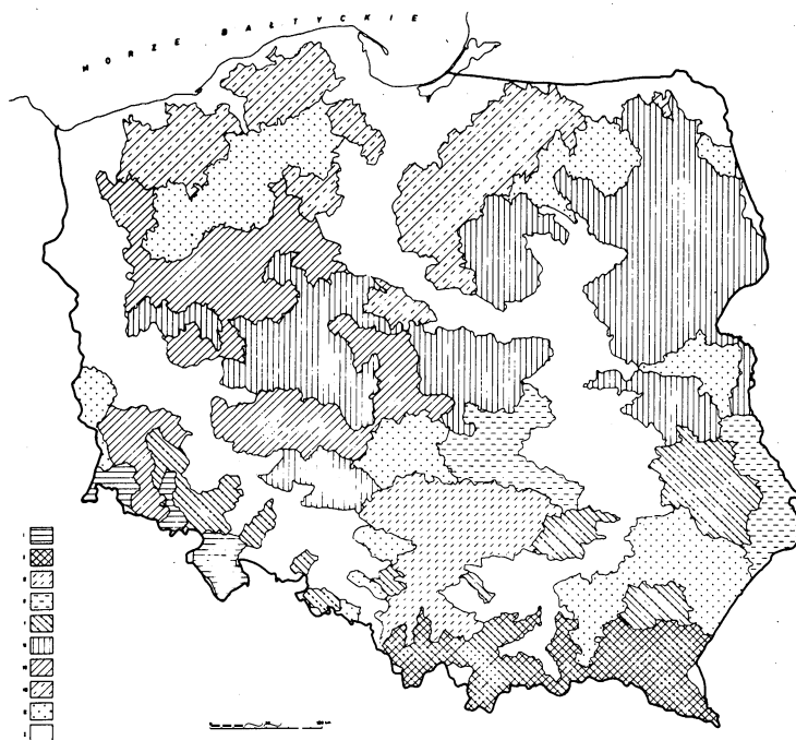
Fig. 1. Catchment basin types.
