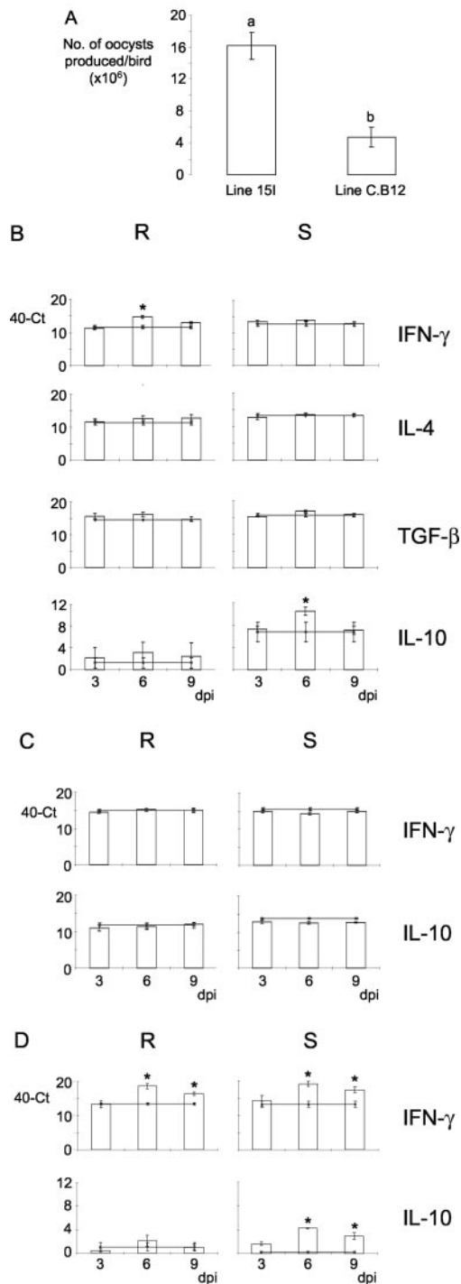
FIGURE 7. Cytokine mRNA expression patterns correlate with susceptibility to infection with E. maxima . A , Total oocyst output in resistant (line C.B12) and susceptible (line 15I) chickens. Different letters indicate values that differ significantly at p < 0.05 . Cytokine mRNA expression was determined in the spleen ( B ), cecal tonsil ( C ), and small intestine ( D ) of resistant line C.B12 (R) and susceptible line 15I (S) chickens at 3, 6, and 9 dpi with E. maxima . Bars indicate cytokine levels in infected chickens on each of the days. Lines indicate levels in age-matched uninfected chickens at 6 dpi. *, Values differ significantly at p < 0.05 .
