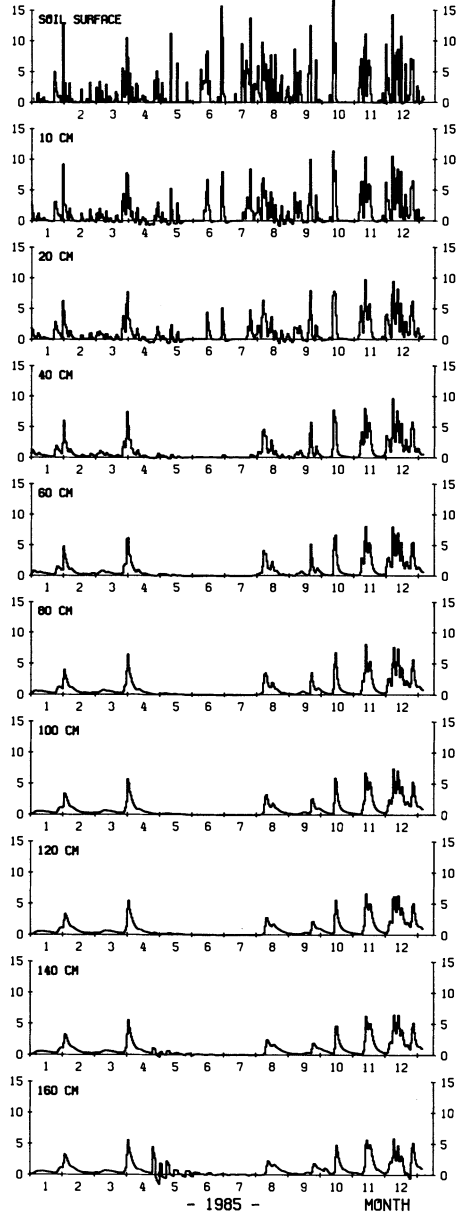
Fig. 14. Jynde vad (profile C1). Simulated water flow (Darcy).
