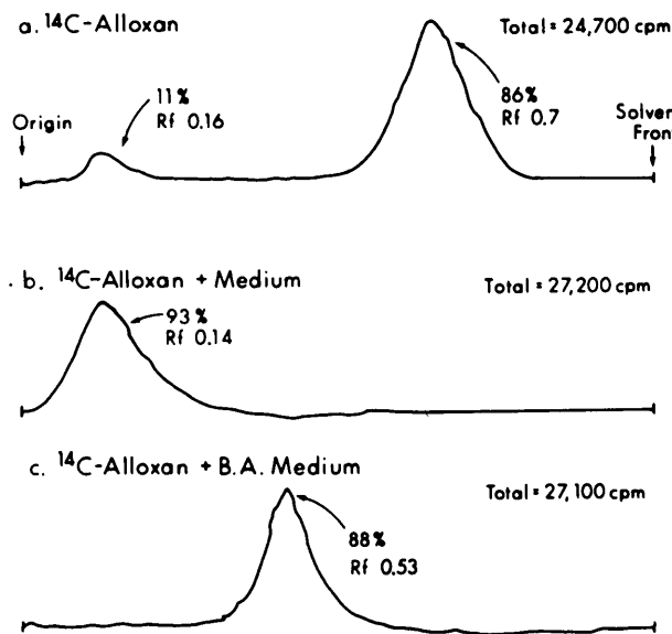
FIG. 6. The reaction between ( ^{14} C) alloxan (650 \mu M, 3.0 mCi/mmol) and 20 mM barbituric acid (B.A.). Shown are tracings of radiochromatograms from thin-layer chromatographic (TLC) plates that contained the following: (a) 5 \mu l. of ( ^{14} C) alloxan (650 \mu M) in 1 mM HCl, (b) 5 \mu l. of ( ^{14} C) alloxan incubated for five minutes at 37° C. and pH 7.4 in 100 \mu l. of Krebs-Ringer medium, (c) 5 \mu l. of ( ^{14} C) alloxan incubated for five minutes at 37° C. in 100 \mu l. of medium supplemented with 20 mM barbituric acid. Final quantitation of the radioactivity associated with each plate was obtained by liquid scintillation counting of sections of the TLC plate.
