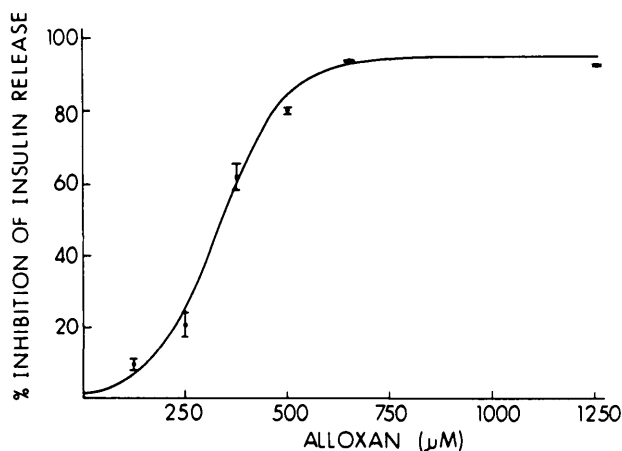
FIG. 2. The effect of alloxan concentration on glucose-induced insulin release. Islets in the experimental group were exposed to alloxan for five minutes at 37^\circ\ \text{C} ., the medium was removed, and the islets were then incubated in glucose ( 27.5\ \text{mM} ) medium for 30 minutes at 37^\circ\ \text{C} . The insulin release from the alloxan-treated islets was compared with that from parallel, untreated groups of islets (mean rate, 3.99\ \mu\text{U} . per islet per minute). Mean \pm S.E.M. N=8-12 . The curve was machine-generated from least-squares analysis ( r = 0.9903 ). Per cent inhibition = [(untreated rate minus alloxan-treated rate) divided by (untreated rate)] times 100 per cent.
