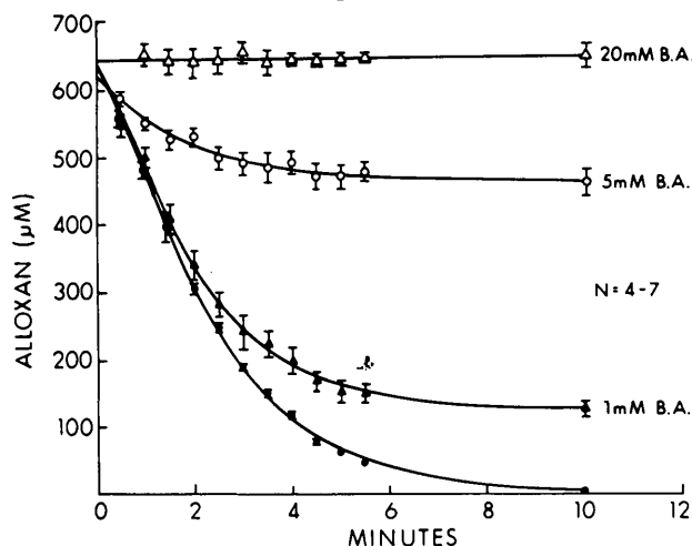
FIG. 5. The decomposition of alloxan (650 \mu M) in the presence ( \Delta , \circ , \square ) and absence ( \bullet ) of barbituric acid (B.A.). Alloxan was added to 10 ml. of Krebs-Ringer medium with and without barbituric acid (1, 5, and 20 mM) at pH 7.4 and 37° C. Portions (4-20 \mu l.) of the reaction mixture were removed at 0.5-minute intervals and assayed fluorometrically for alloxan (see MATERIALS AND METHODS). Mean \pm S.E.M. The curves were machine-generated from least-squares analysis.
