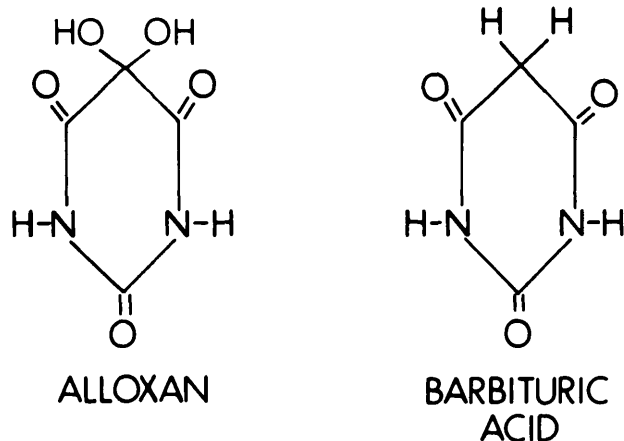
FIG. 1. Chemical structures of alloxan (hydrated form) and barbituric acid.
