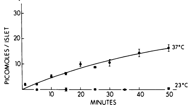
FIG. 4. Time study of barbituric acid uptake. Islets were incubated for the indicated intervals in 100 \mu l. of medium containing ( ^{2-14} C) barbituric acid (20 mM, 0.56 mCi./mmol) and ( ^3 H) sucrose (20 mM, 1.5 mCi./mmol) at 37° C. or 23° C. Curve was machine-generated from least-squares analysis. N=4-6 .
