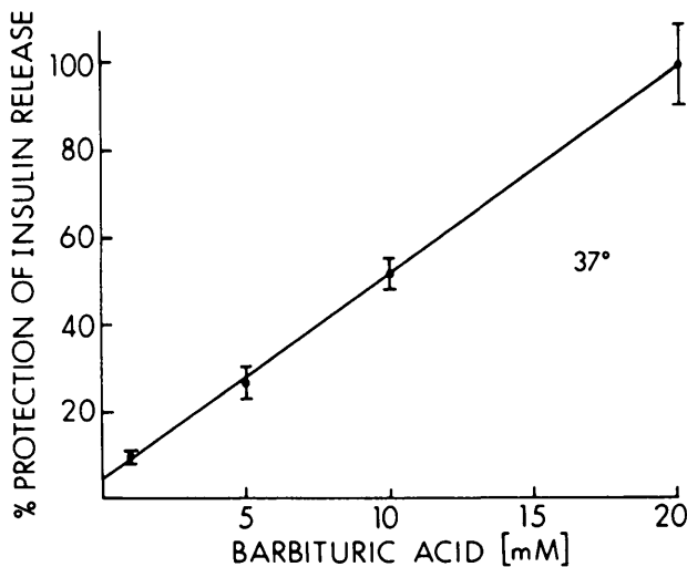
FIG. 3. Barbituric acid protection against alloxan inhibition of glucose-induced insulin release. Islets were exposed to alloxan (650 \mu M) for five minutes at 37° C. in the presence of barbituric acid and then stimulated with glucose medium as in figure 2. Insulin release from alloxan-treated islets was compared with that from parallel groups of untreated islets (mean rate, 2.84 \mu U. per islet per minute). Mean \pm S.E.M. The line was drawn from linear least-squares analysis ( r = 0.9997 ). N=9-15 . Per cent protection = [(alloxan-treated rate minus basal rate) divided by (untreated rate minus basal rate)] times 100 per cent.
