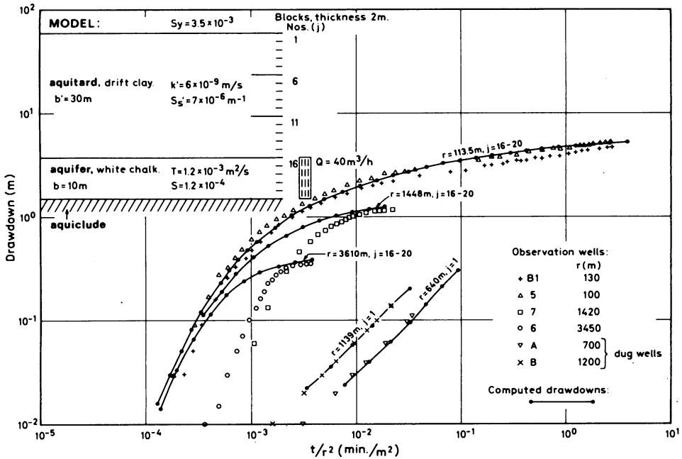
Fig. 6. Observed and modelled drawdowns versus t/r^2 during pumping test on well 3, Torkildstrup-Lillebrænde Waterworks, Falster, Denmark. Test reported by Kærgaard (1980).
