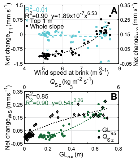
Figure 6. A: Rate of net surface height change (including grainfall and grainflow affected areas) for each scan period for both the top 1 \text{ m} of the lee slope (T1) and the entire lee slope (WS), as a function of wind speed. B: Rate of net surface height change across the entire lee slope as a function of maximum grainfall length ( GL_{95} , bottom x axis) and saltation flux at the brink (saltation flux, Q_{Sz} , top x axis).
