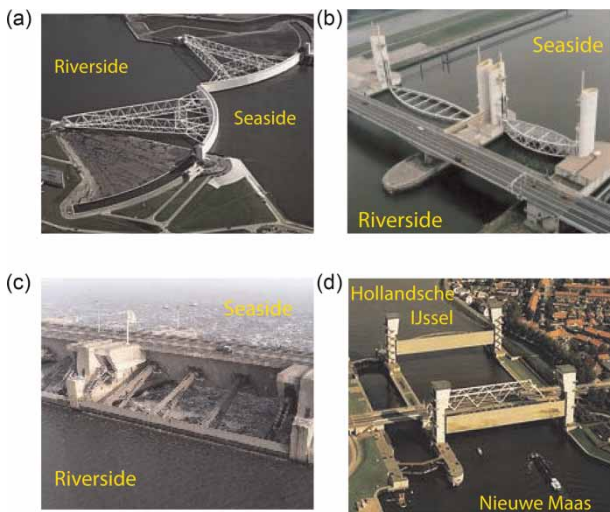
Figure 2 | Storm surge barriers in the Rhine–Meuse delta (van Overloop 2009). (a) Maeslant barrier, (b) Hartel barrier, (c) Haringvliet sluices and (d) Hollandsche IJssel barrier.
