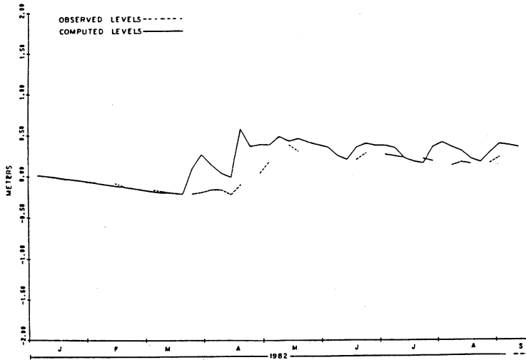
Fig. 8. Lake Laflamme watershed: observed and computed levels at piezometer 3.
