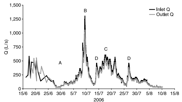
Figure 7 | Seasonal stream flow pattern of Black Top Ridge Creek (BTRC), 2006. Here A refers to a low stream flow period, B indicates the flood event from the release of a snow dam, C indicates melt from late-lying snow beds and D indicates stream flow peaks driven by rain and melt generated from rain on snow.
