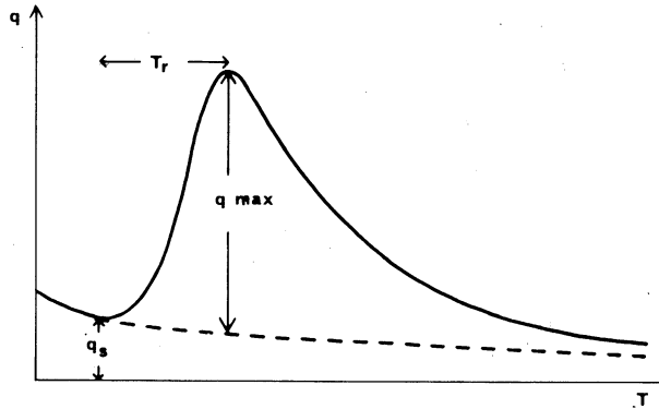
Fig. 3. Selected characteristics on a flood hydrograph.
