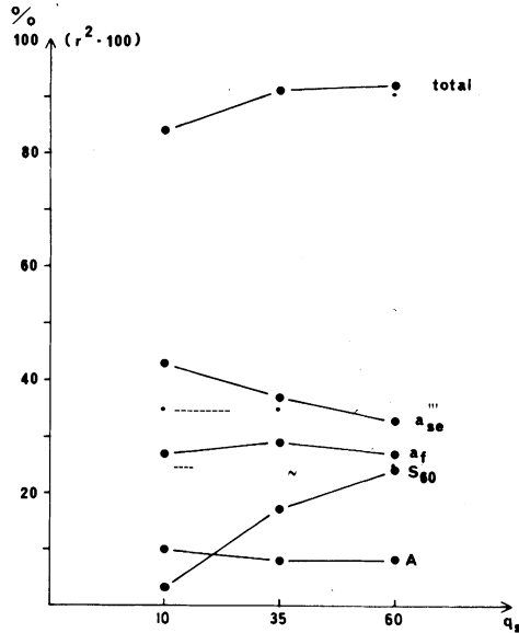
Fig. 5. Change in the watershed characteristics' contribution to peak runoff q_{\max} as a function of start runoff q_s while basin rainfall P_e and rainfall intensity I_e are held constant like 15 mm respectively 3 mm/hour.
