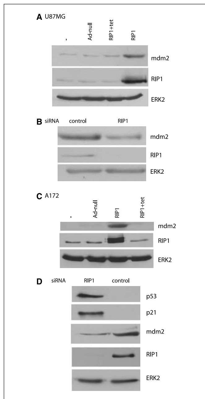
Figure 2. RIP1 regulates mdm2 levels. A , increased expression of RIP1 leads to up-regulation of mdm2 levels in U87MG cells. Ad-RIP1 was introduced into cells for 24 h followed by lysate preparation and Western blot. Adenovirus-null and RIP1 + tetracycline were used as negative controls. B , siRNA knockdown of RIP1 results in a decrease in mdm2 levels in U87MG cells compared with control (scrambled, nonsequence) siRNA, as shown in the Western blot. C , increased expression of RIP1 up-regulates mdm2 in A172 cells. The experiment was performed as described for A . D , siRNA knockdown of RIP1 results in a decrease in mdm2 levels in A172 cells compared with control (scrambled, nonsequence).
