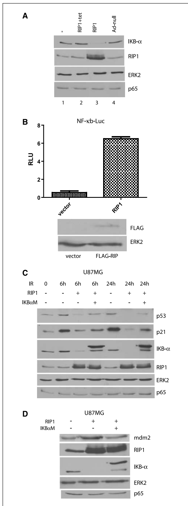
Figure 3. A, introduction of Ad-RIP1 into U87MG cells results in down-regulation of IκBα, which indicates NF-κB activation. Lysates were prepared 24 h after RIP1 infection and adenovirus-null and RIP1 + tet were used as negative controls. B, U87MG cells were transfected with an NF-κB-responsive promoter linked to luciferase (κB-LUC) and cotransfected with FLAG-RIP1 or empty vector. Whereas the activity of the reporter is low in the vector-transfected cells, introduction of RIP1 results in a strong activation of the transcriptional activity of NF-κB. Bottom, expression of FLAG-RIP1 was confirmed by Western blot with FLAG antibodies. C, a dominant-negative IκBα super-repressor mutant blocks the effect of RIP1 on p53 and p21 induction in response to IR. U87MG cells were infected with Ad-RIP1 + Ad-null or Ad-RIP1 + Ad-IκBαM for 24 h followed by IR for 6 or 24 h and Western blot for p53, p21, IκBα, p65, and RIP1 expression. D, a dominant-negative IκBαM blocks the effect of RIP1 on mdm2 up-regulation. U87MG cells were infected with Ad-RIP1 + Ad-null or Ad-RIP1 + Ad-IκBαM for 24 h followed by Western blot for mdm2. Expression of IκBαM blocks the RIP1-mediated increase in mdm2. Western blots were also probed for the p65 subunit of NF-κB.
