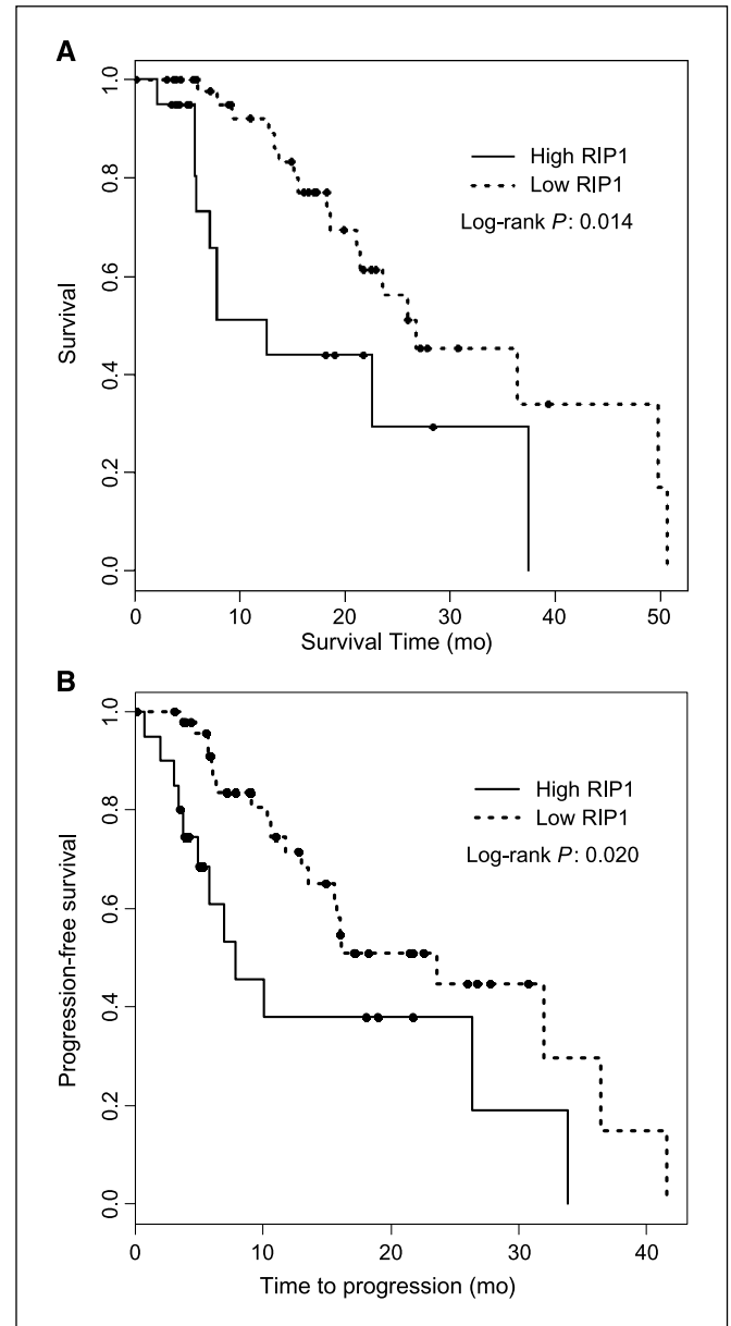
Figure 6. A, Kaplan-Meier estimates of overall survival time in glioblastoma patients, grouped by levels of RIP1. The survival time was significantly longer for patients in low-RIP1 group than those in high-RIP1 group. B, Kaplan-Meier estimates of progression-free survival time in glioblastoma patients grouped by RIP1 levels. The progression-free survival time was significantly shortened for patients who had increased RIP1 levels.
