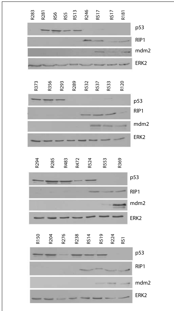
Figure 5. RIP1 levels correlate with mdm2 in glioblastoma. A panel of 31 glioblastomas was tested for mdm2 expression using mdm2 (2A10) antibodies. ERK2 was used to determine loading. The same lysates were also probed for RIP1 and p53. Mdm2 is detectable in ~30% of tumors and strongly correlates with RIP1 levels. An inverse correlation between mdm2 and p53 was also detected.
