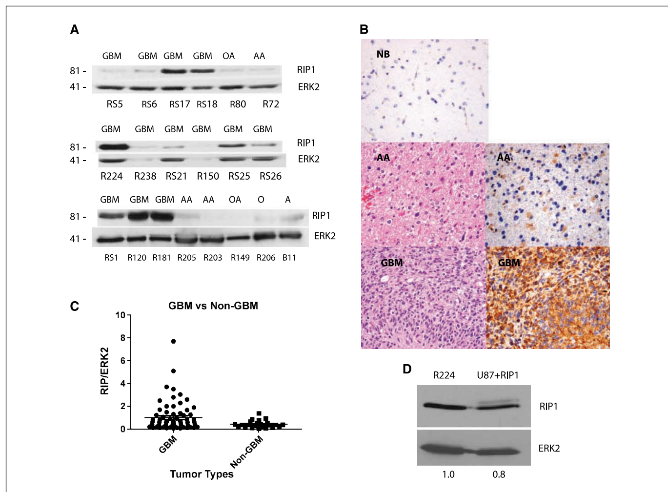
Figure 4. RIP1 expression in glioma. A , Western blots using lysates made from resected tumors. Glioblastomas (GBM; grade IV gliomas) include RS5, RS6, RS17, RS18, R224, R238, RS21, R150, RS25, RS26, RS1, R120, and R181. Nonglioblastomas (grades II–III gliomas) include R80 (OA), R72 (AA), R205 (AA), R203 (AA), R149 (OA), R206 (O), and B11 (A). B , immunohistochemistry of paraffin-embedded sections. NB, normal brain with absent or low RIP1; AA, anaplastic astrocytoma (R72) with H&E staining (left) and a low level of RIP1 staining (right) in the same section; GBM, glioblastoma (R224) with H&E staining (left) and intense RIP1 staining (right) in this tumor. C , levels of RIP1 in glioblastomas versus nonglioblastoma (grades II–III glioma) tumors. The comparison of RIP1 level between 70 glioblastoma samples and 23 nonglioblastoma samples shows that RIP1 level correlates with increased malignancy. D , level of RIP1 overexpression achieved by infecting U87MG cells with adenoviral RIP1 (MOI, 50) is similar to expression levels in high RIP1-expressing glioblastomas (R224 is shown here). Protein (10 \mu g) was loaded followed by Western blot with RIP1 antibodies. AO, anaplastic oligodendroglioma; AOA, anaplastic oligoastrocytoma; AA, anaplastic astrocytoma; OA, oligoastrocytoma; O, oligodendroglioma; A, astrocytoma.
