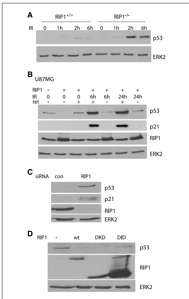
Figure 1. RIP1 regulates p53 levels. A , Western blot showing p53 induction at various times in RIP1 -/- primary MEFs compared with wild-type MEFs in response to IR (10 Gy). The Western blot was probed with p53 antibodies (1C12). ERK2 was used as a loading control. B , U87MG cells were infected with RIP1 adenovirus (MOI, 50) in a tet-off system followed by IR (10 Gy) and preparation of lysates as indicated. As a control, tetracycline ( tet , 1 μg/mL) was added with RIP1 virus to prevent RIP1 expression. Western blots were probed with a p53 (DO1) and p21 antibodies. Increased RIP1 blocks p53/p21 induction in response to radiation. C , U87MG cells were transfected with control or RIP1 siRNA. At 72 h later, lysates were prepared followed by Western blot. Loss of RIP1 augments p53 and p21 levels. Similar results were obtained with two other RIP1 siRNA oligos. D , U87MG cells were infected with wild-type or mutant RIP1 for 24 h and then followed by Western blot. DKD , deletion of kinase domain; DID , deletion of intermediate domain. Center , expression of the RIP1 wild-type ( upper band ) and truncated mutants ( lower band ).
