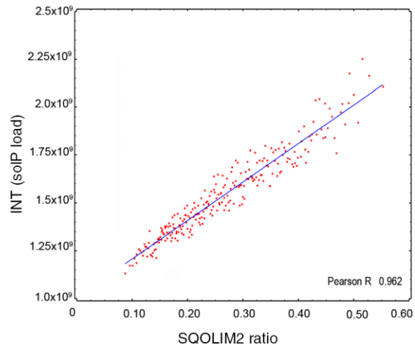
Figure 8 | Scatter plot showing the most important input-output relationship based on stepwise regression, case study 1.
