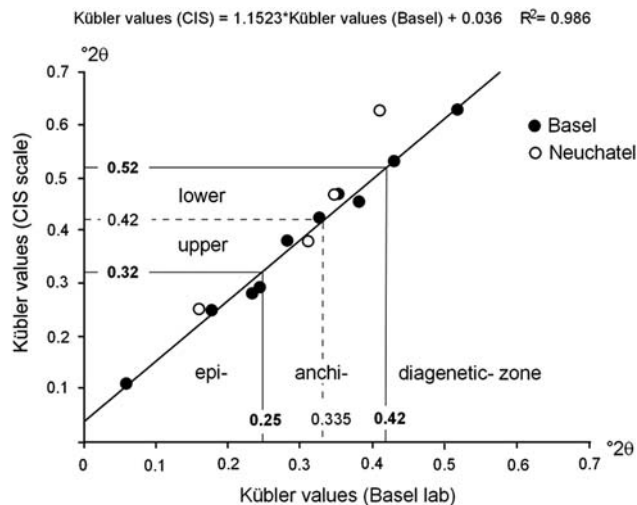
FIG. 1. Correlation plot of Kübler Index values determined using the CIS scale and the experimental values provided by the laboratories of Basel (M. Frey and W.B. Stern) and Neuchâtel (Kübler and coworkers). Kübler's anchizone limits of 0.25°2 \theta and 0.42°2 \theta , translate into 0.32°2 \theta and 0.52°2 \theta for the CIS scale based on the Basel correlation.
