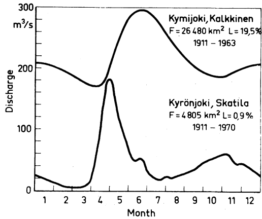
Fig. 1. Mean discharge in a big river with high lake percentage, and in a small river with low lake percentage.
