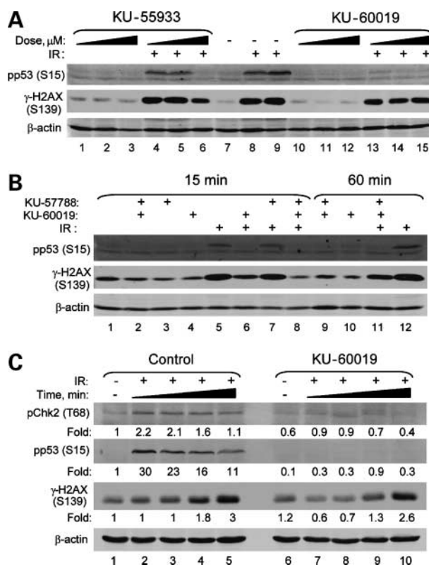
Figure 2. KU-60019 is a more effective inhibitor of the ATM kinase than is KU-55933. A , U87 cells were treated with KU-55933 or KU-60019 (0, 1, 3, or 10 \mu mol/L) for 1 h, exposed to 10 Gy of ionizing radiation and collected for Western blot analysis after 1 h. B , U87 cells were treated with KU-57788 (2.5 \mu mol/L), KU-60019 (3 \mu mol/L), or both, exposed to 10 Gy of ionizing radiation, and collected for Western blot analysis after 15 or 60 min. C , U1242 cells were treated with KU-60019 (3 \mu mol/L), exposed to 5 Gy, and collected for Western blot analysis after 5, 15, 30, or 60 min. Fold depicts phospho-protein levels normalized to \beta -actin levels. Drugs remained in the medium throughout the experiments.
