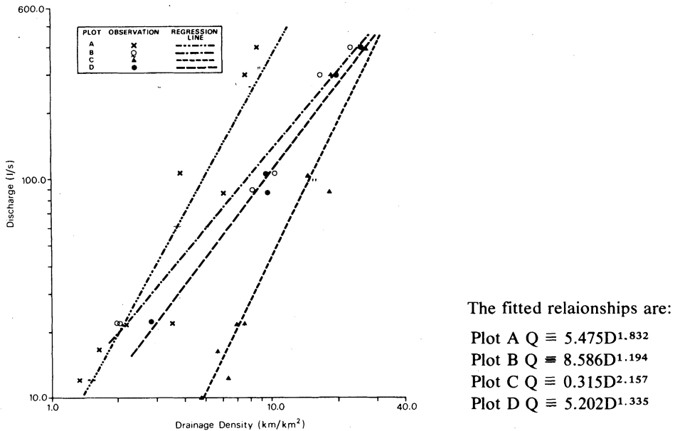
Fig. 11. The relationship between catchment discharge and drainage density within plots covered by vegetation of varying composition.
