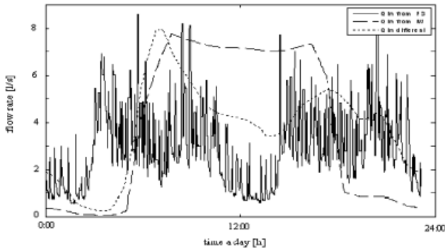
Figure 3 | Different inflow patterns – Qin base inflow pattern (dashed line), more representative inflow pattern of a domestic dominated catchment (dotted line) and inflow data from a flow survey (solid line).
