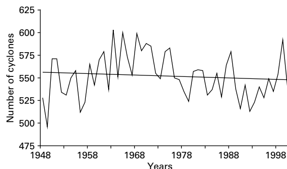
Figure 3 Time series of the number of cyclones in the Atlantic–European sector (30°W–45°E, 35–75°N)
