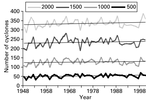
Figure 4 Time series of the number of cyclones in the circles with the radius of 500, 1000, 1500 and 2000 km centred on the point 60°N, 22.5°E
