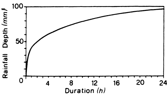
Fig. 7. Rainfall depth-duration curve for a 25-year return period. Raingauge of Cortona (see Fig. 1).
