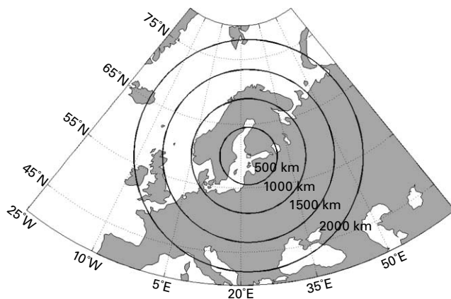
Figure 1 Location map of the Atlantic–European sector and the circles with radii of 500, 1,000, 1,500 and 2,000 km centred in 60°N, 22.5°E
