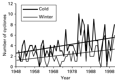
Figure 9 Time series of the frequency of long-term cyclones moving in the zone B–B in winter and in the cold half-year
