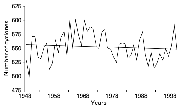
Figure 3 Time series of the number of cyclones in the Atlantic–European sector (30°W–45°E, 35–75°N)
