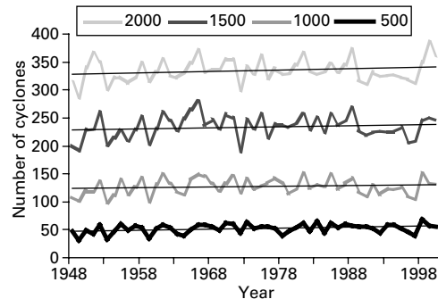
Figure 4 Time series of the number of cyclones in the circles with the radius of 500, 1000, 1500 and 2000 km centred on the point 60°N, 22.5°E
