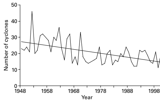
Figure 7 Time series of the annual number of cyclones in zone C
