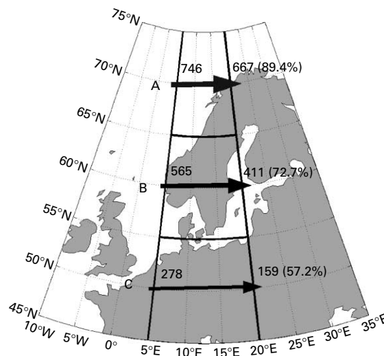
Figure 8 Number of long-term cyclones crossing 5°E and 20°E at the zones A, B and C
