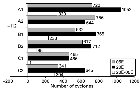
Figure 5 Number of cyclones that crossed the meridians 5°E and 20°E by the sub-zones during the period 1948–2000 and the difference between the number of cyclones that crossed 20°E and 5°E
