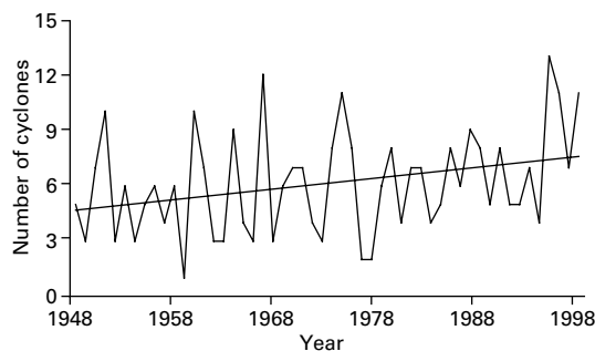
Figure 6 Time series of the number of cyclones crossing sub-zone B1 (60–65°N) of the 20°E meridian in winter
