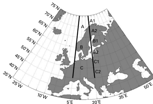
Figure 2 Location map of the area around meridians 5°E and 20°E with zones A, B, C and their sub-zones
