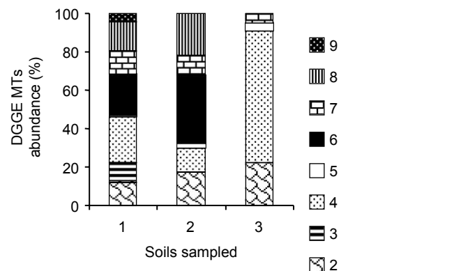
Figure 5 | Presence and percentage of DGGE MTs of uidA PCR products at the different soils sampled: S1 produced MT2 to MT9; S2 produced MT2, MT4, MT5, MT6, MT7 and MT8; and S3 produced MT2, MT4, MT5 and MT7.
