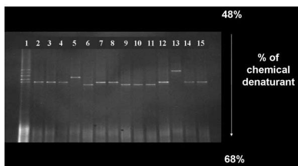
Figure 1 | Syber-Green staining of a parallel DGGE gel of E. coli soil isolates by PCR amplification of \beta -D-glucuronidase gene fragment (uidA) using primer pair UAL-1939GC and UAL-2105. Lane 1, MTs from different E. coli water isolates used in each DGGE as control. Lanes 2 to 15, E. coli isolates collected at a depth of 0 to 5 cm from soil 1 (S1) at time 3 (T3).
