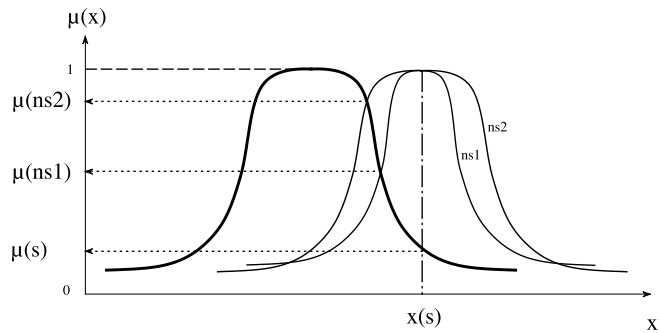
Figure 10 | Fuzzification of two fuzzy numbers (ns1 and ns2) with different standard deviations (SD of ns2>SD of ns1) and one crisp number x(s) which is also the most probable value for the fuzzy numbers.
