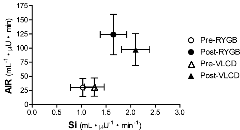
FIG. 2. Graphic representation of the relationship between insulin sensitivity and insulin secretion before and after interventions.
