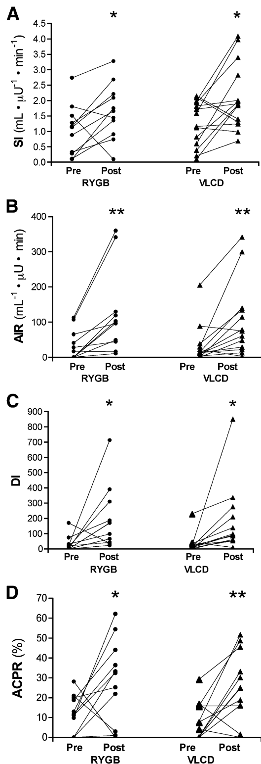
FIG. 1. Changes in S_i (A), AIR (B), DI (C), and ACPR (D) for all subjects shown individually. * P < 0.05 , ** P < 0.01 , *** P < 0.001 vs. baseline.
