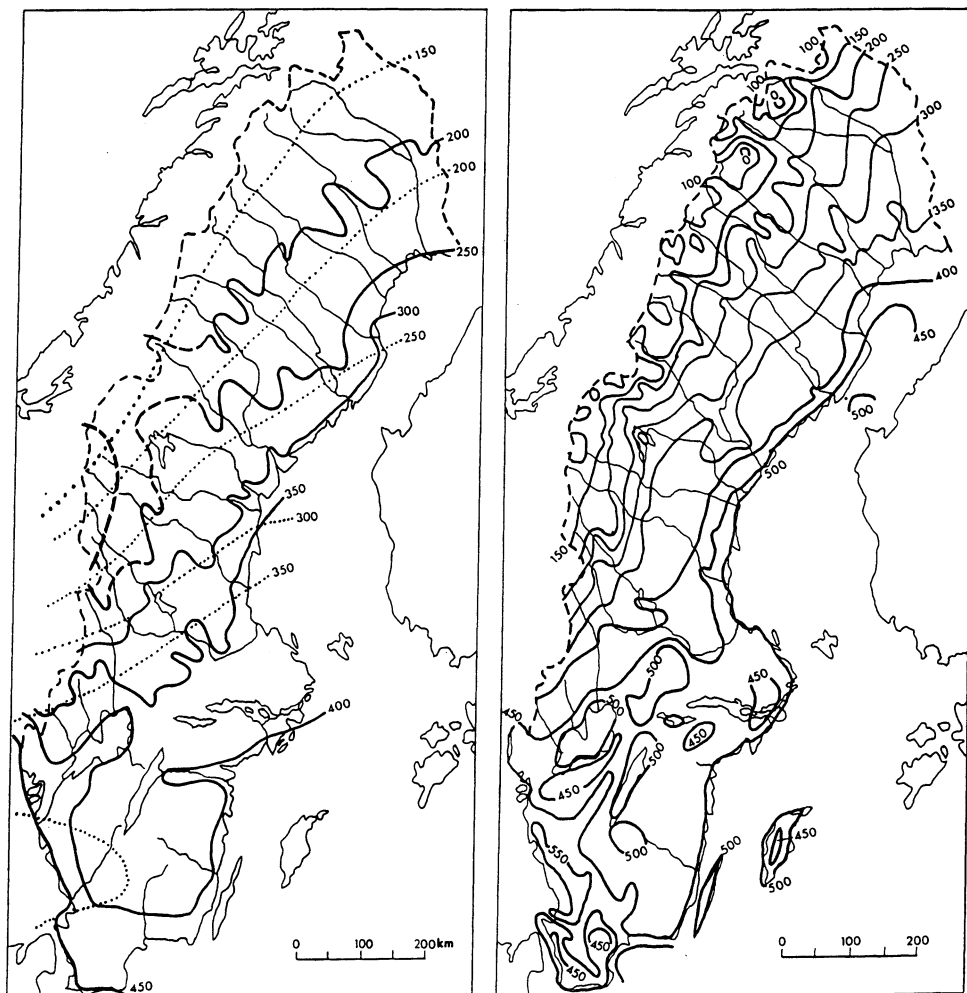
Fig. 1a. Actual evaporation (mm/year) over Sweden calculated as a residual water balance term. The left map, redrawn from Tamm (1959), shows results by Bergsten (1954) as dotted isolines and by Tamm (1954) as solid isolines. Both authors based their calculations on data from 1921-1950 and did not correct for precipitation errors. The right map, redrawn from Eriksson (1980a), is based on data from the period 1931-1960 and on corrected precipitation records.
