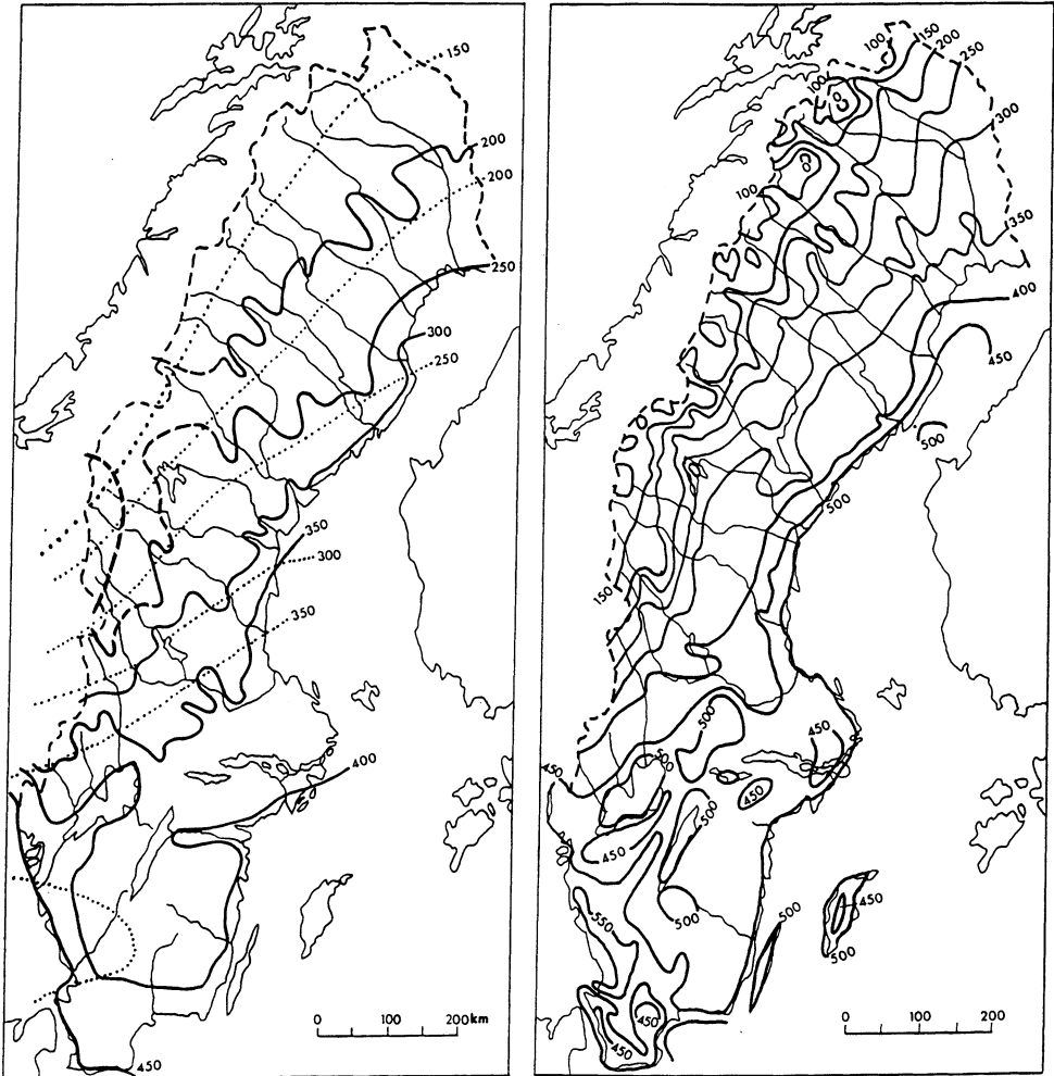
Fig. 1a. Actual evaporation (mm/year) over Sweden calculated as a residual water balance term. The left map, redrawn from Tamm (1959), shows results by Bergsten (1954) as dotted isolines and by Tamm (1954) as solid isolines. Both authors based their calculations on data from 1921-1950 and did not correct for precipitation errors. The right map, redrawn from Eriksson (1980a), is based on data from the period 1931-1960 and on corrected precipitation records.
