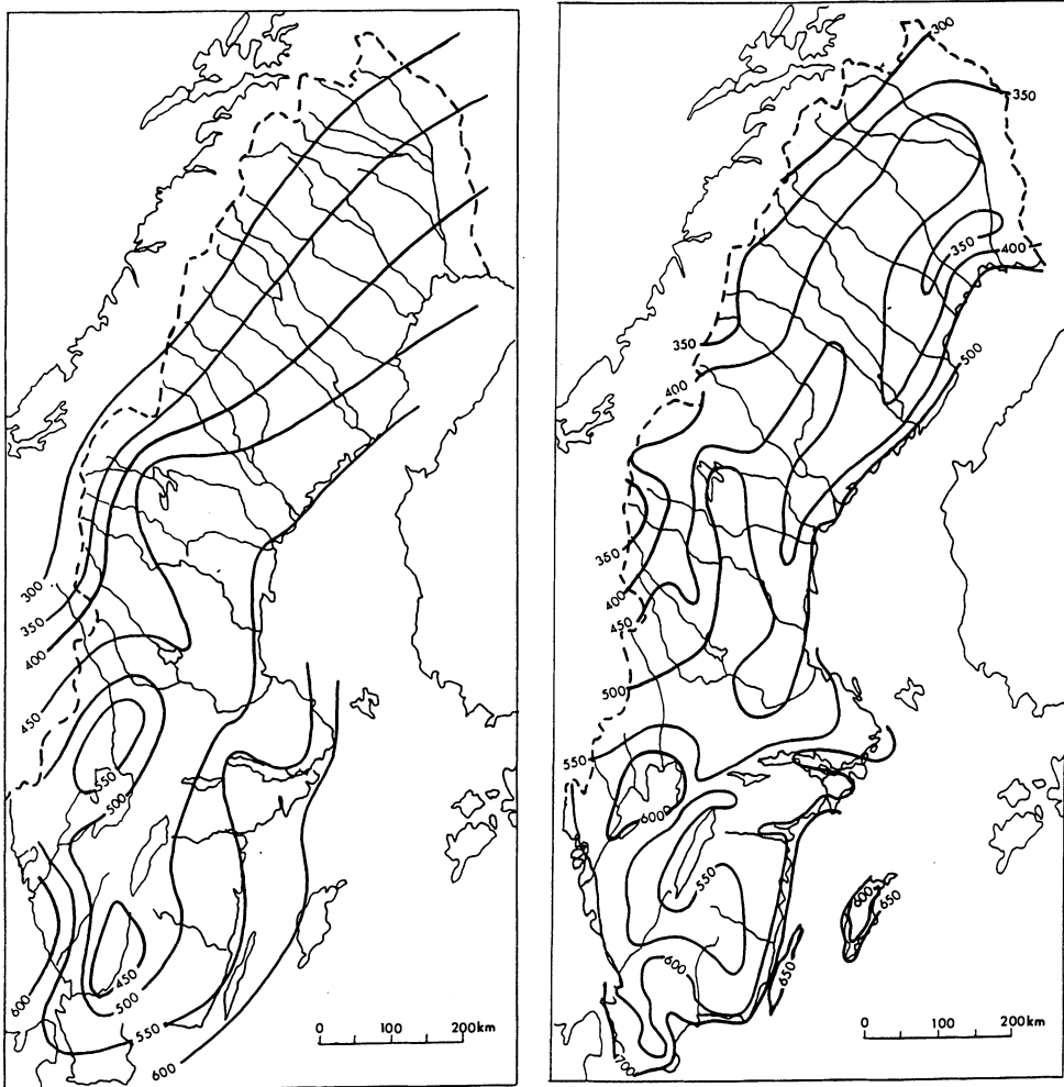
Fig. 1b. Potential evaporation (mm/year) over Sweden calculated with the Penman (1948) formula. The left map, redrawn from Wallén (1966), is based on data from the period 1931-1960, whereas the right map, redrawn from Eriksson (1981), is based on data from the period 1961-1978.
