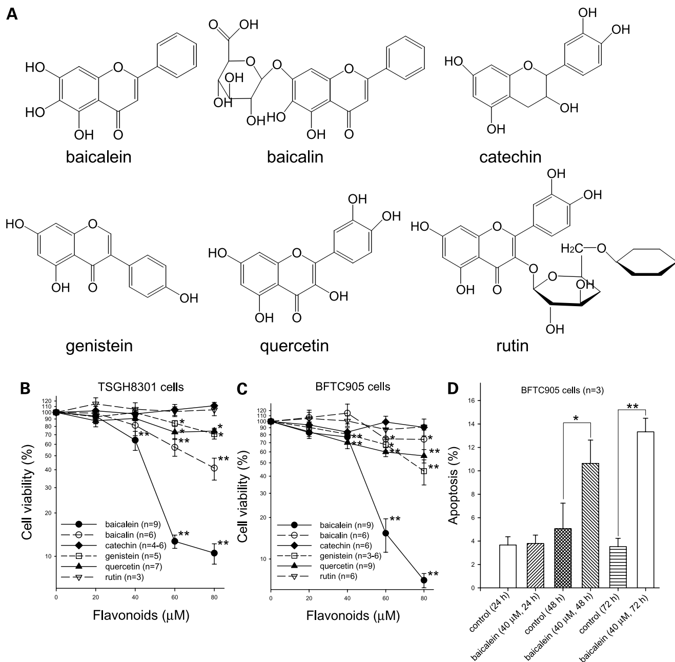
Figure 1. Effects of baicalin on the cytotoxicity and apoptosis in bladder cancer cells. A , chemical structures of flavonoids. B and C , TSGH8301 or BFTC905 cells were treated with 0 to 80 \mu M baicalin, baicalin, catechin, genistein, quercetin, and rutin for 24 h. After drug treatment, the cells were recultured for 2 d. The cell viability was measured by MTT assay. Points, mean; bars, SE. *, P < 0.05 ; **, P < 0.01 , significant difference between control and flavonoid-treated samples. D , the cells were treated with or without 40 \mu M baicalin for 24 to 72 h. The percentage of apoptosis was scored by the apoptotic nuclei under a fluorescence microscope. Results were obtained from three experiments. Columns, mean; bars, SE. *, P < 0.05 ; **, P < 0.01 , significant difference between control and baicalin-treated samples.
