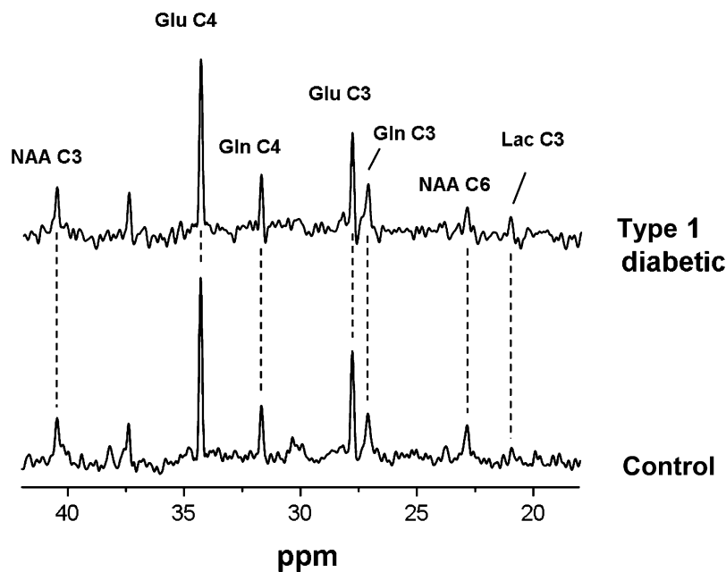
FIG. 3. ^{13}\text{C} MR spectra of a T1D subject ( top ) and control subject ( bottom ) averaged over the last 30 min of [3\text{-}^{13}\text{C}] lactate infusion.
