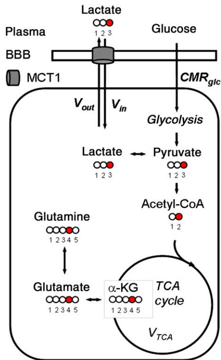
FIG. 2. One-compartment model describing incorporation of ^{13}\text{C} label from [3-^{13}\text{C}] lactate into the brain glutamate and glutamine pools. This figure illustrates the fluxes V_{in} (lactate influx), V_{out} (lactate efflux), CMR_{glc} (glucose consumption), and V_{TCA} (TCA cycle rate), which were considered to derive Eq. 2. BBB, blood-brain barrier; \alpha -KG, \alpha -ketoglutarate; MCT1, MCA transporter 1. ●, ^{13}\text{C} -labeled carbon position. Lactate in the neuronal and glial compartments was treated as a single pool due to the rapid transfer of lactate between these cells (24).
