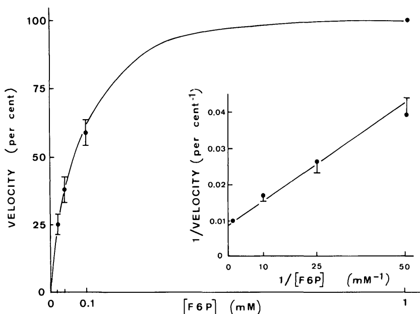
FIGURE 1. Saturation curve and double reciprocal plot for the activity of fructose-6-P,2-kinase at increasing concentrations of fructose-6-P. The velocity of the reaction is expressed as a percent of the paired value found within the same experiment in the presence of 1.0 mM fructose-6-P. Such a control value averaged 79.6 \pm 9.1 fmol/min per islet (N = 14). Mean values ( \pm SEM) refer to 6–8 individual observations.
