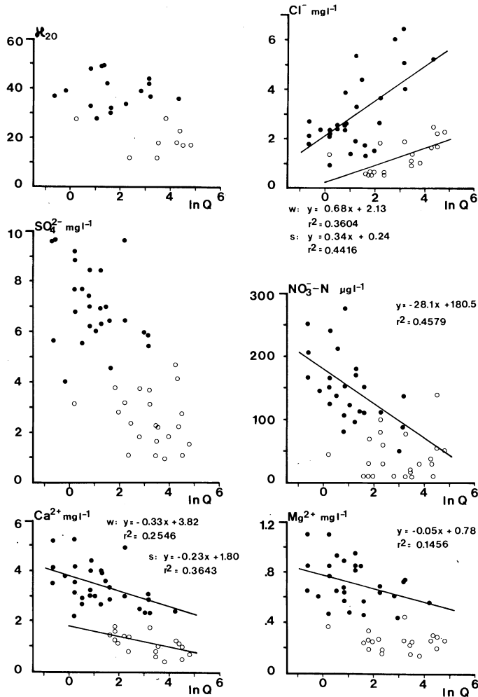
Fig. 5. The relation between specific conductance, concentrations of major ions and the water discharge. Only significant regression lines are drawn ( p < 0.05 ). s and open circles denote summer season, whereas w and black circles denote winter season. Q is the water discharge.
