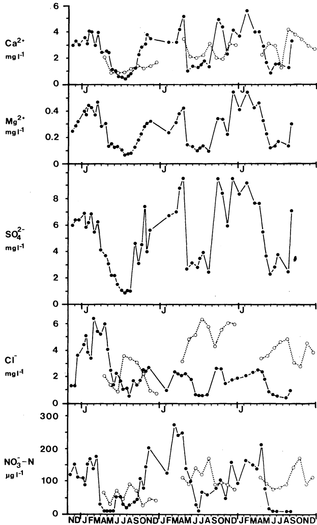
Fig. 4. Concentrations of major ions at the inlet of the weir basin at Ekse from Nov. 75 to Sep. 78. Open circles denote concentrations found at Ekse during 1967, 68, and 69.
