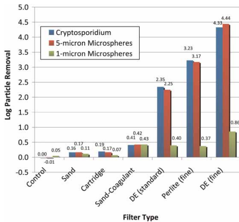
Figure 4 | Log particle removal for each filtration scenario.
