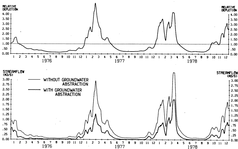
Fig. 5. Streamflow depletions in Køge Å caused by an additional groundwater abstraction of 10 mm/year (upper figure) and 200 mm/year (lower figure) within Køge Å catchment. All the streamflows are 15 days' moving average values.
